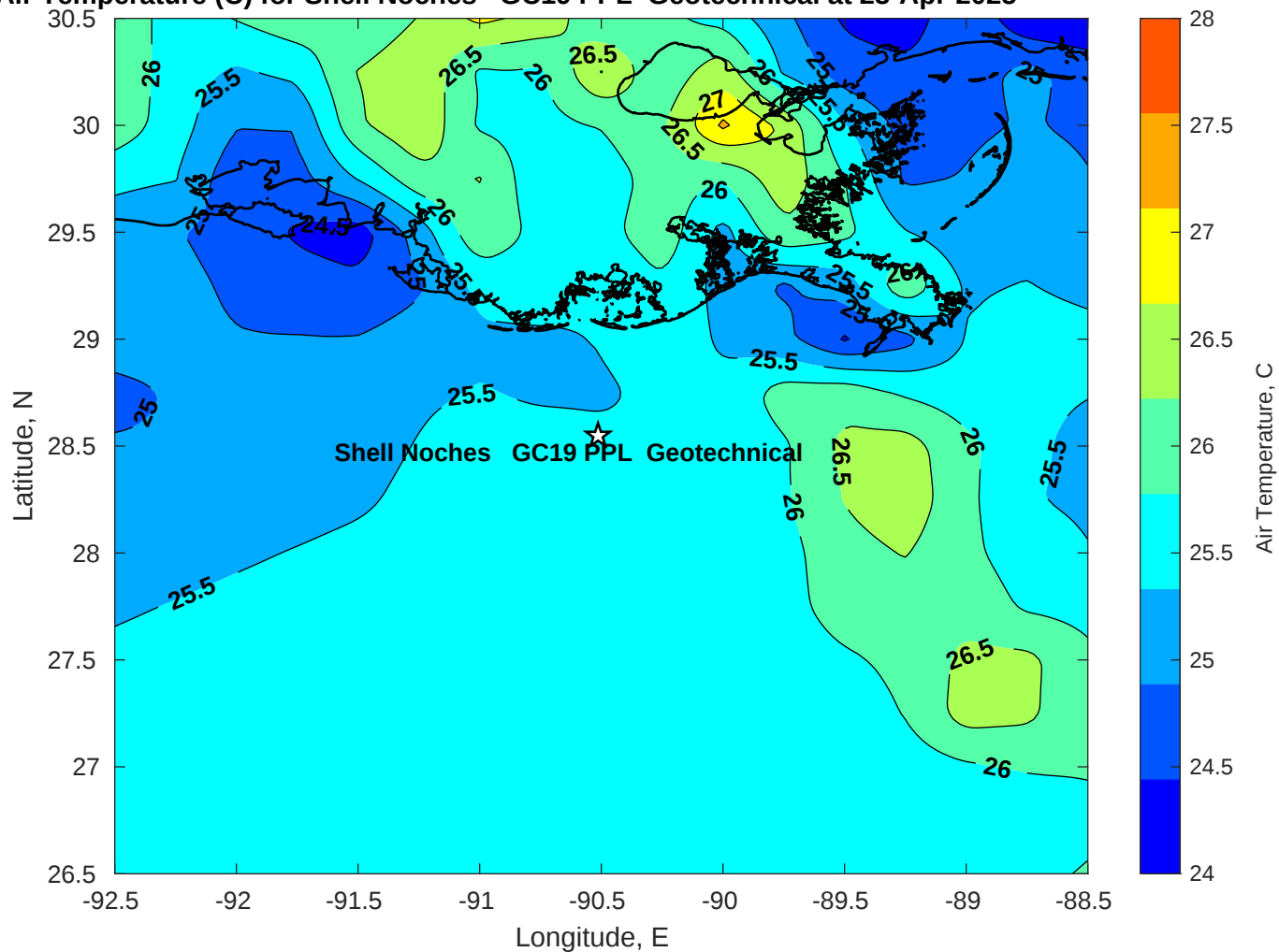
Air Temperature (C) for Shell Noches GC19 PPL Geotechnical at 23-Apr-2025
