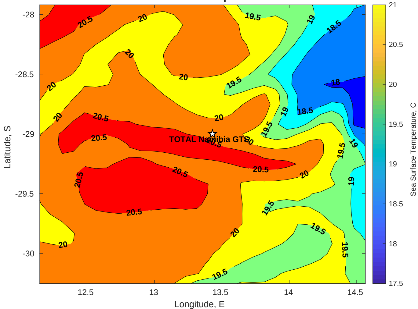
SST for TOTAL Namibia GTS at 22-Apr-2025 00:00:00
