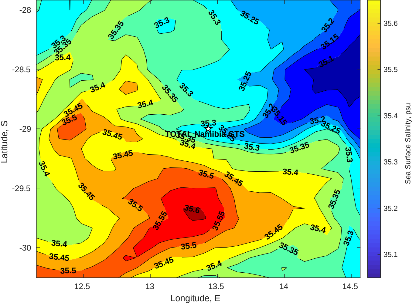
Surface Salinity for TOTAL Namibia GTS at 22-Apr-2025 00:00:00
