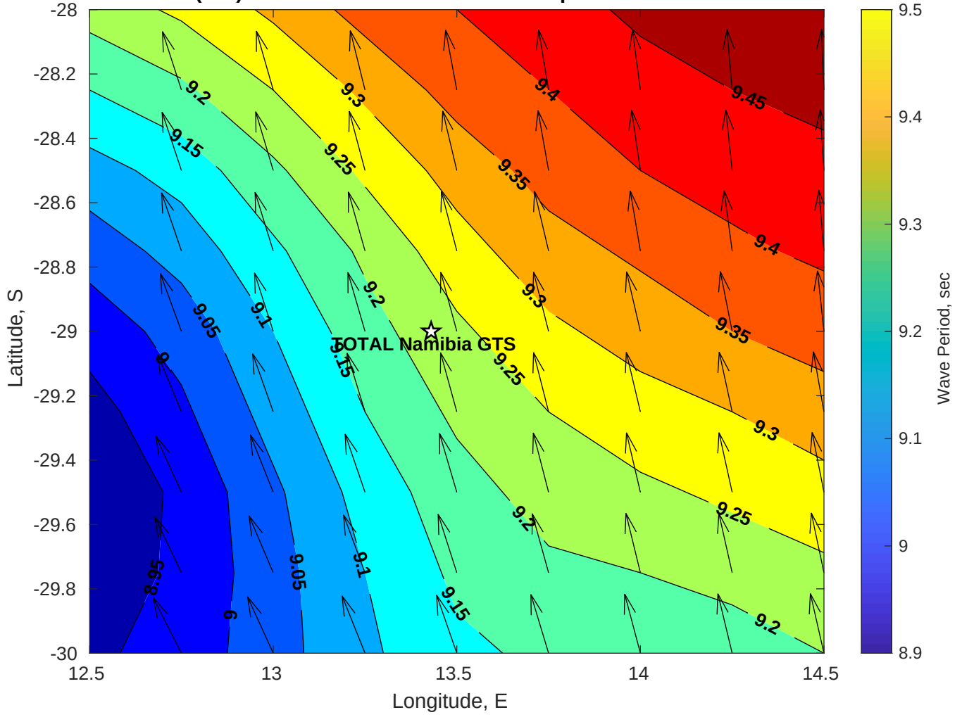
Wave Period (sec) for TOTAL Namibia GTS at 23-Apr-2025 09:00:00
