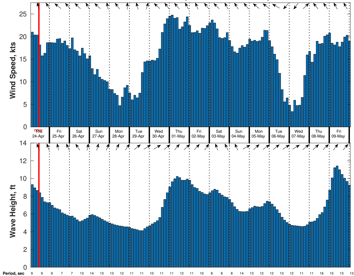
Wind & Wave Forecast for TOTAL Namibia GTS from 23-Apr-2025 02:00:00 to 09-May-2025 02:00:00
