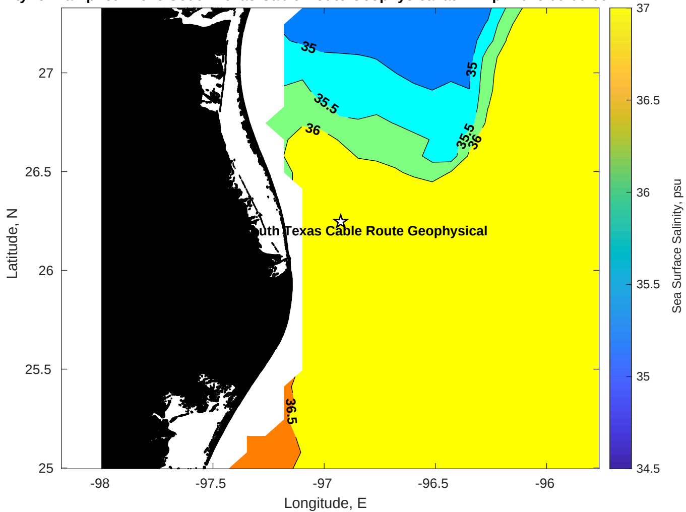
Surface Salinity for Tampnet P2378 South Texas Cable Route Geophysical at 22-Apr-2025 00:00:00
