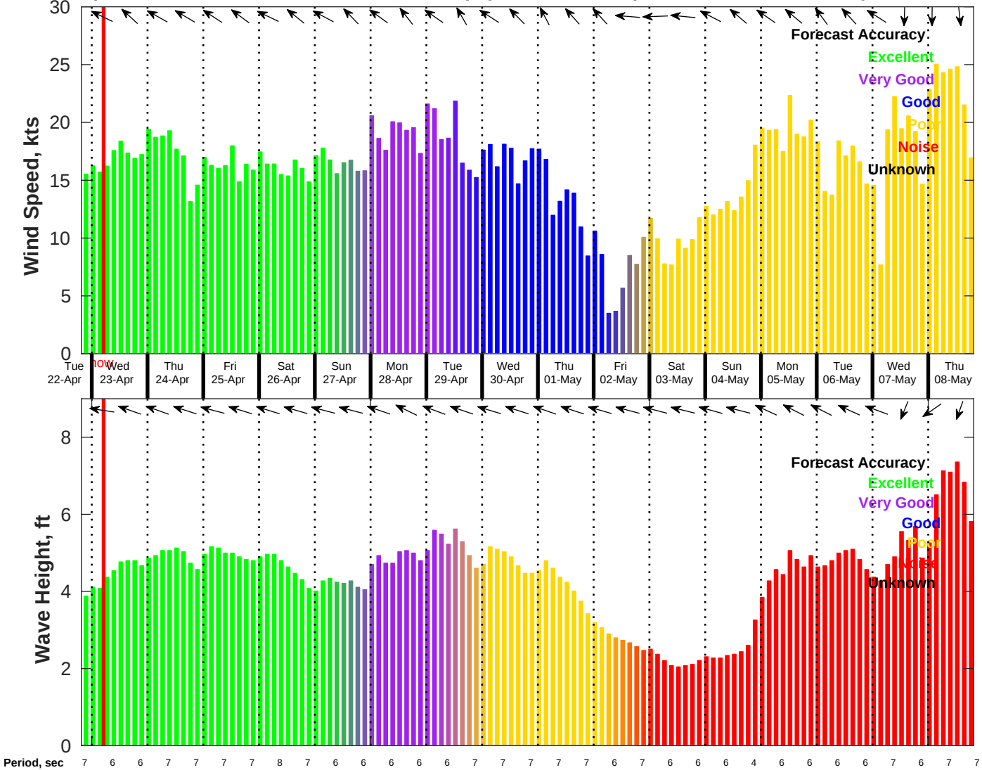
Wind & Wave Forecast for Tampnet P2378 South Texas Cable Route Geophysical from 22-Apr-2025 20:00:00 to 08-May-2025 20:00:00
