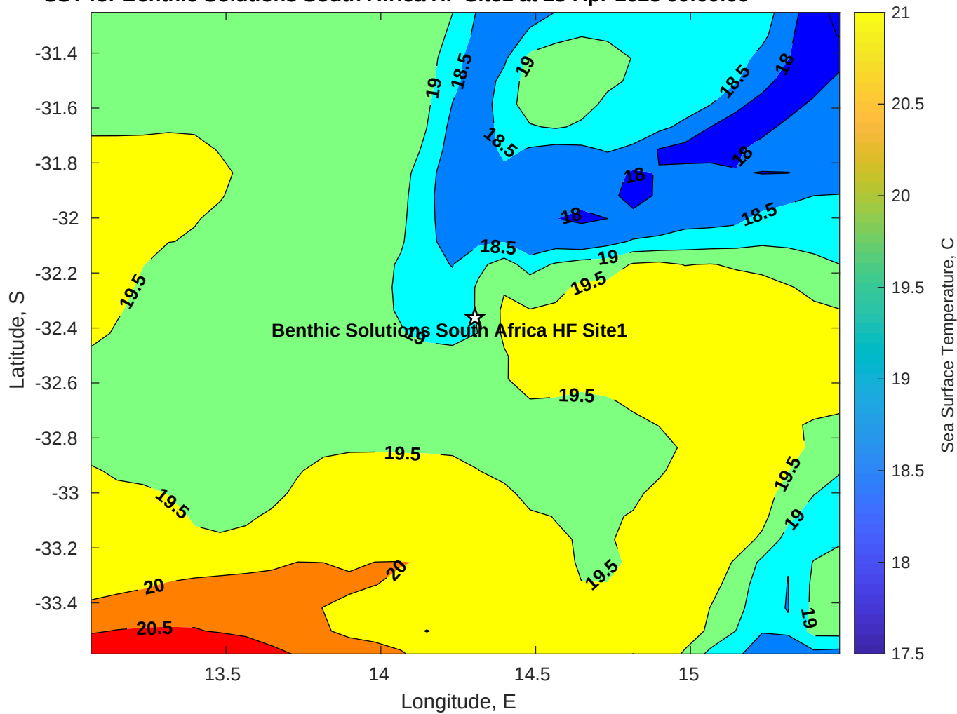
SST for Benthic Solutions South Africa HF Site1 at 23-Apr-2025 00:00:00
