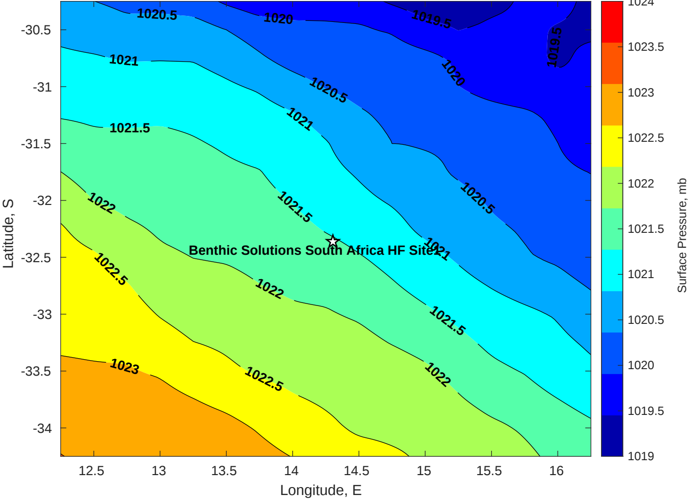
Surface Pressure (mb) for Benthic Solutions South Africa HF Site1 at 24-Apr-2025 00:00:00
