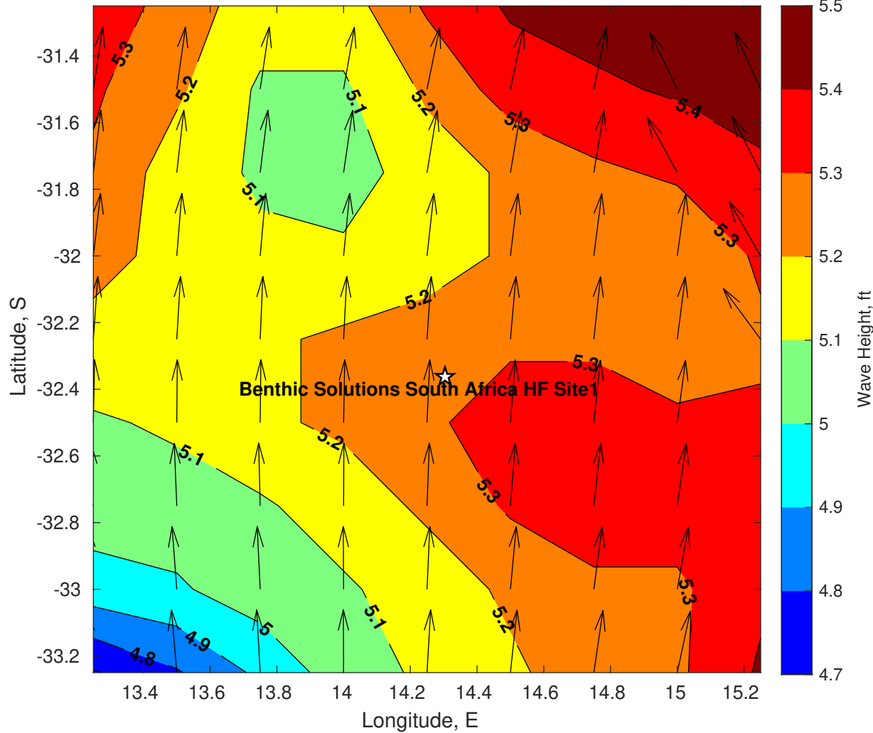
Wave Height (ft) for Benthic Solutions South Africa HF Site1 at 24-Apr-2025 09:00:00
