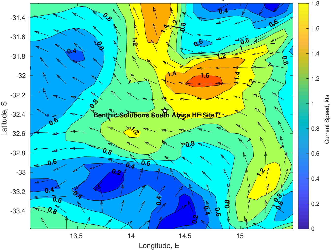
Surface Currents for Benthic Solutions South Africa HF Site1 at 23-Apr-2025 00:00:00
