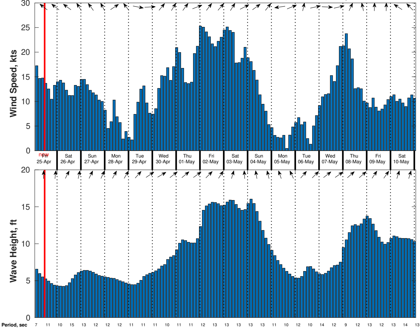
Wind & Wave Forecast for Benthic Solutions South Africa HF Site1 from 24-Apr-2025 02:00:00 to 10-May-2025 02:00:00
