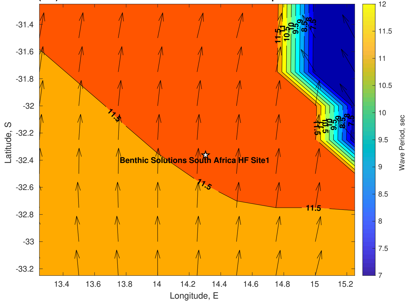
Wave Period (sec) for Benthic Solutions South Africa HF Site1 at 24-Apr-2025 09:00:00
