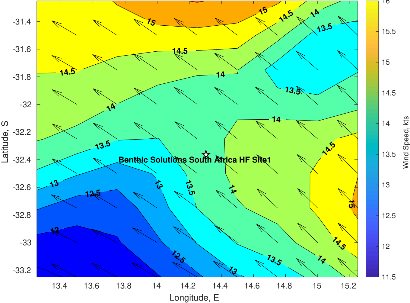
Winds (kts) for Benthic Solutions South Africa HF Site1 at 24-Apr-2025 09:00:00
