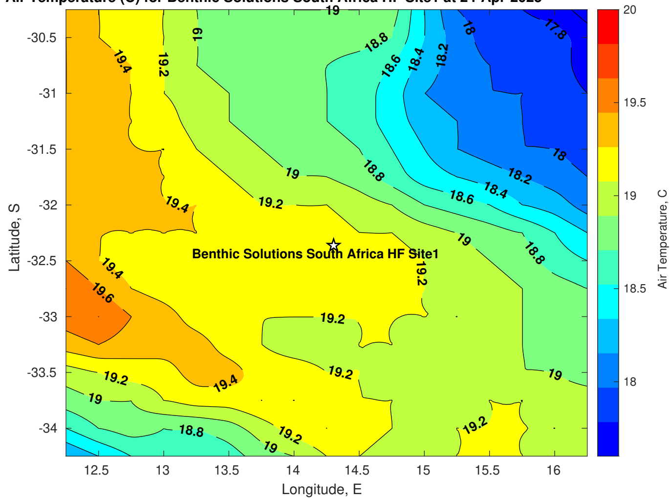
Air Temperature (C) for Benthic Solutions South Africa HF Site1 at 24-Apr-2025
