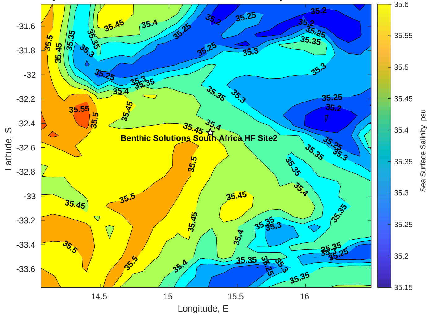
Surface Salinity for Benthic Solutions South Africa HF Site2 at 23-Apr-2025 00:00:00
