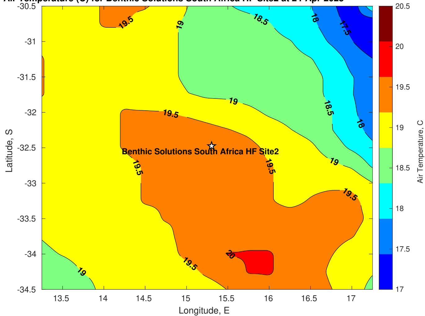
Air Temperature (C) for Benthic Solutions South Africa HF Site2 at 24-Apr-2025
