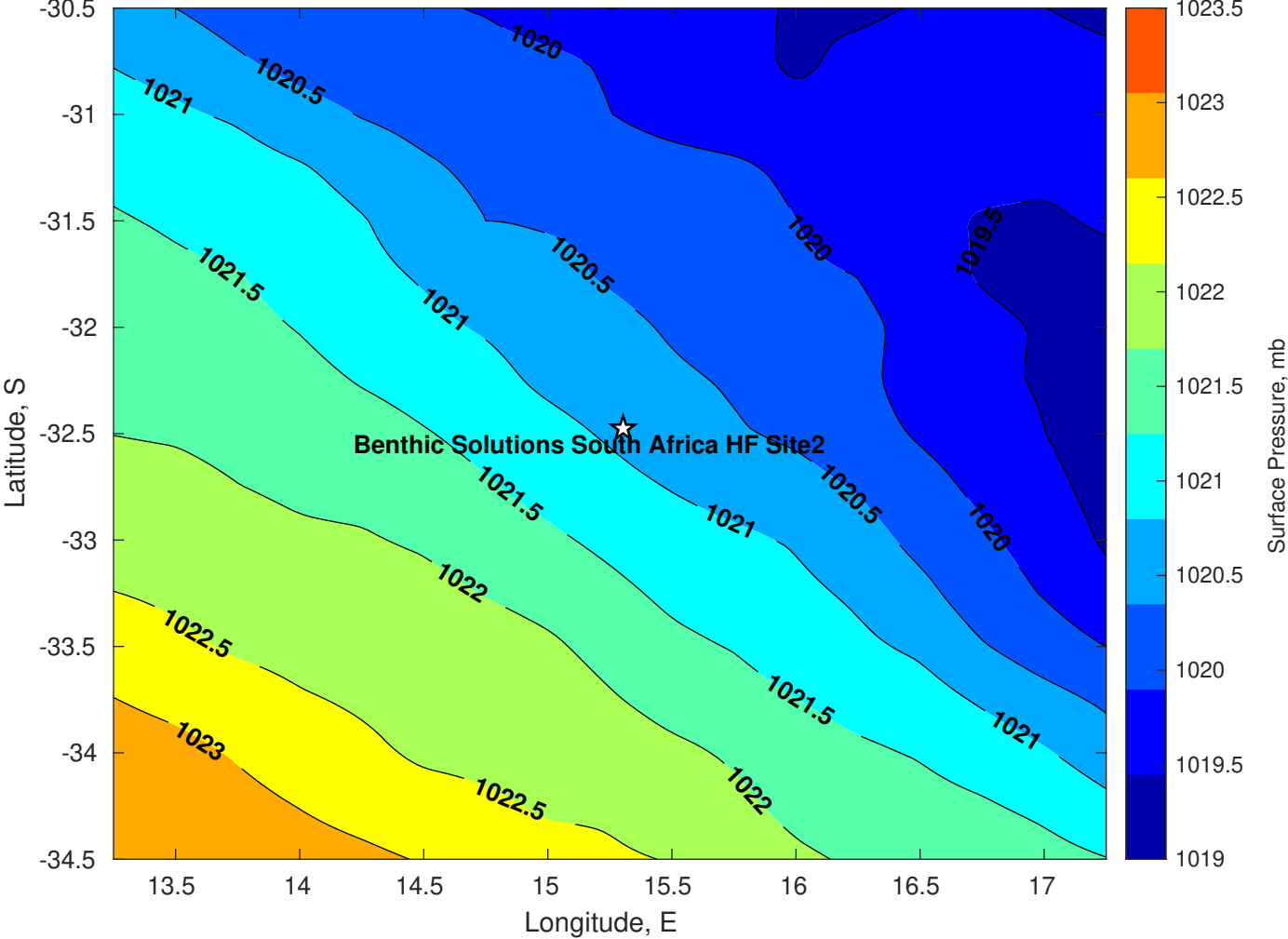
Surface Pressure (mb) for Benthic Solutions South Africa HF Site2 at 24-Apr-2025 00:00:00
