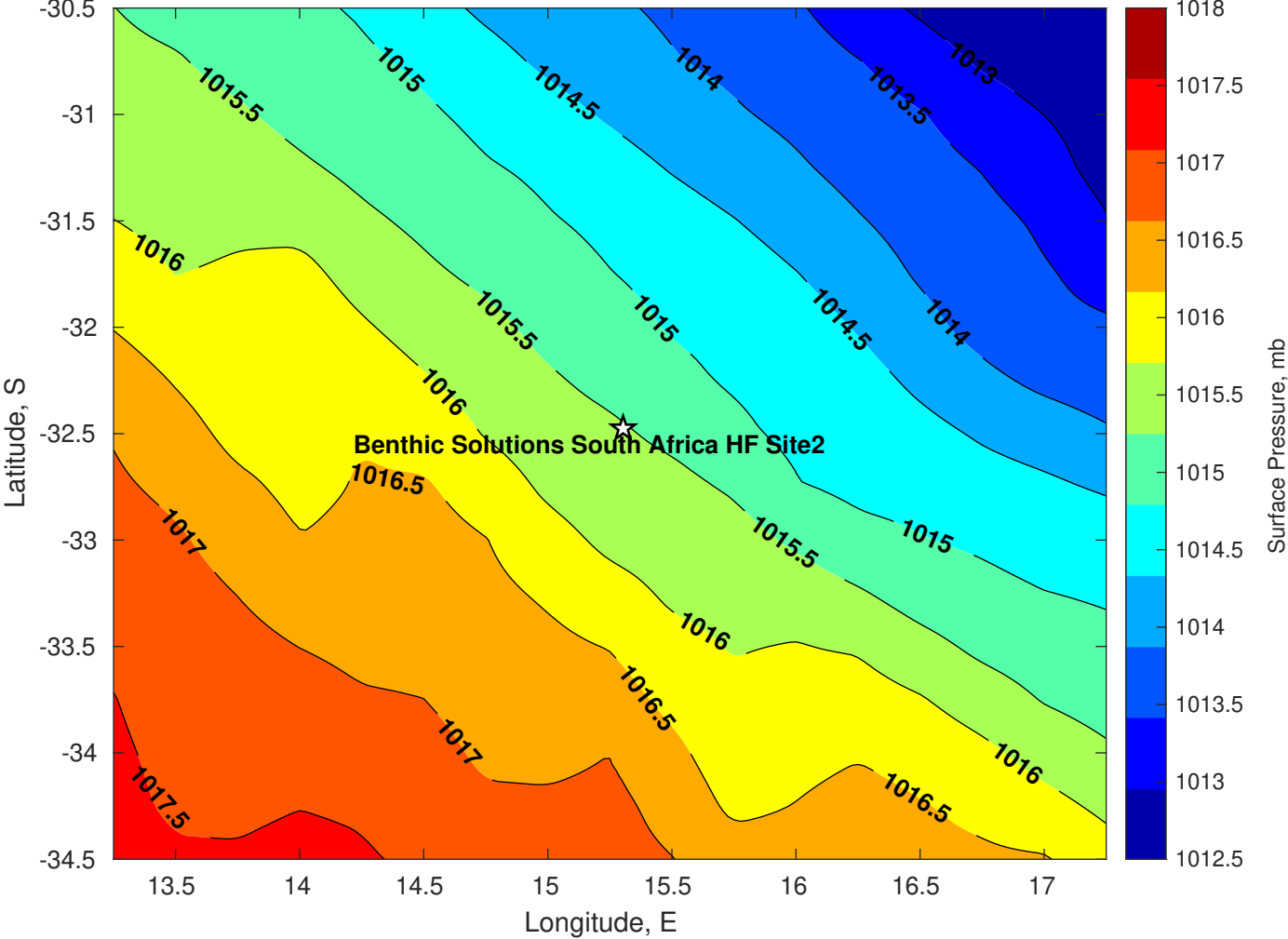
Surface Pressure (mb) for Benthic Solutions South Africa HF Site2 at 26-Apr-2025 00:00:00
