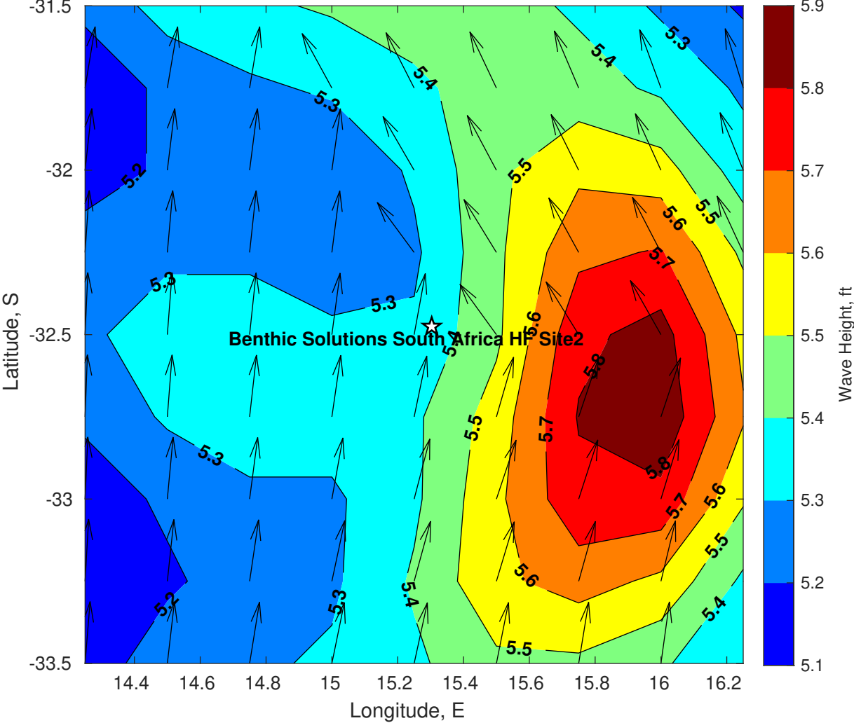
Wave Height (ft) for Benthic Solutions South Africa HF Site2 at 24-Apr-2025 09:00:00
