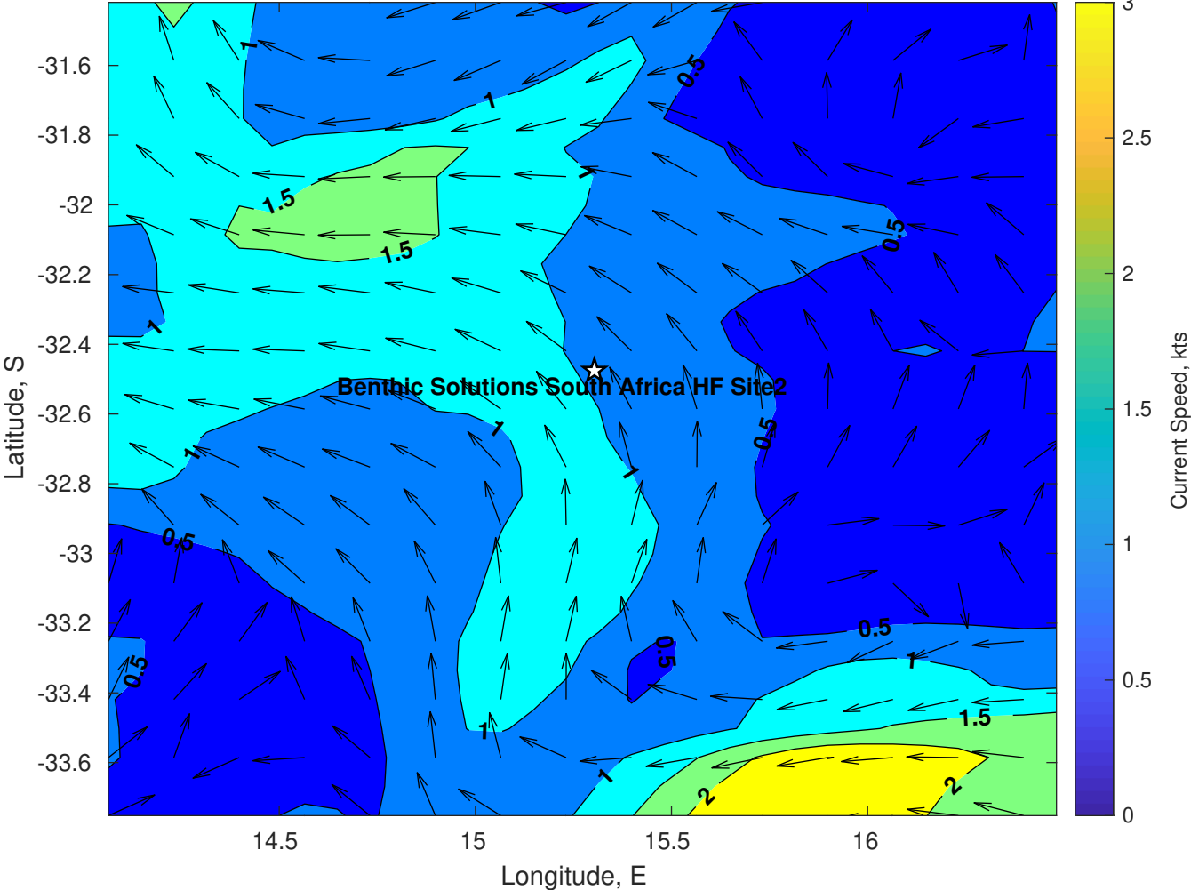
Surface Currents for Benthic Solutions South Africa HF Site2 at 23-Apr-2025 00:00:00
