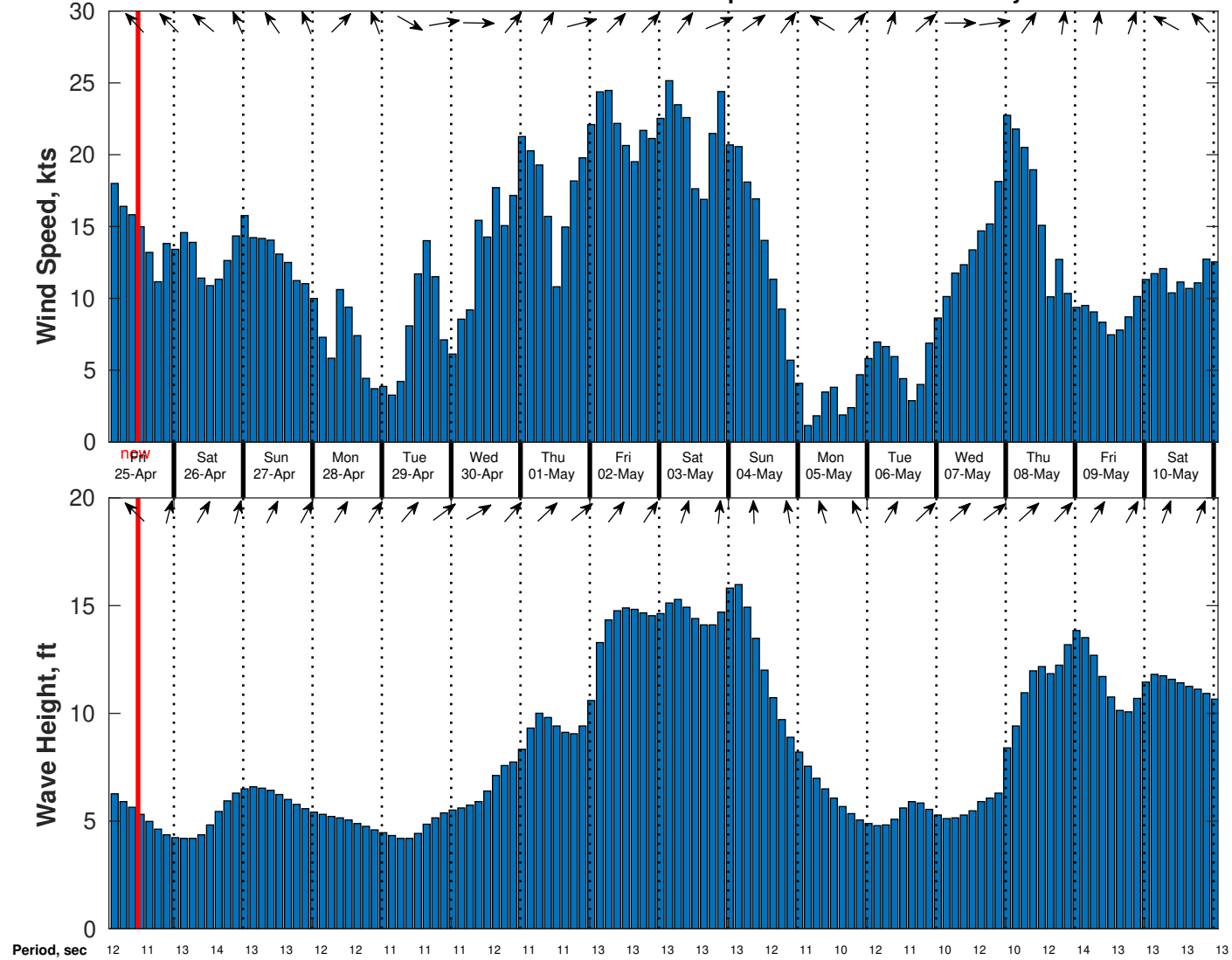
Wind & Wave Forecast for Benthic Solutions South Africa HF Site2 from 24-Apr-2025 02:00:00 to 10-May-2025 02:00:00
