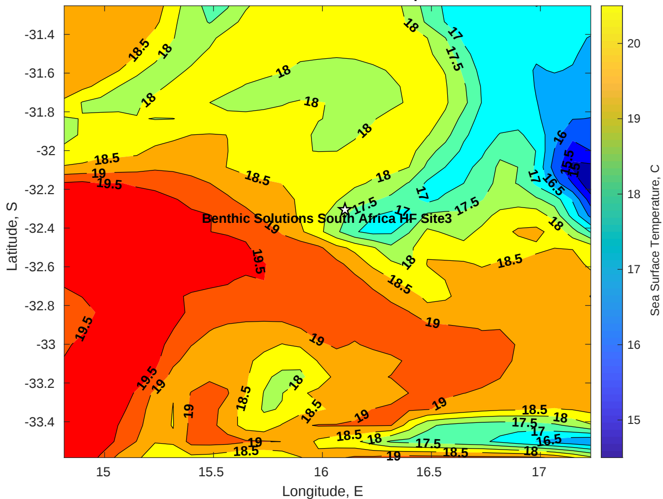
SST for Benthic Solutions South Africa HF Site3 at 23-Apr-2025 00:00:00
