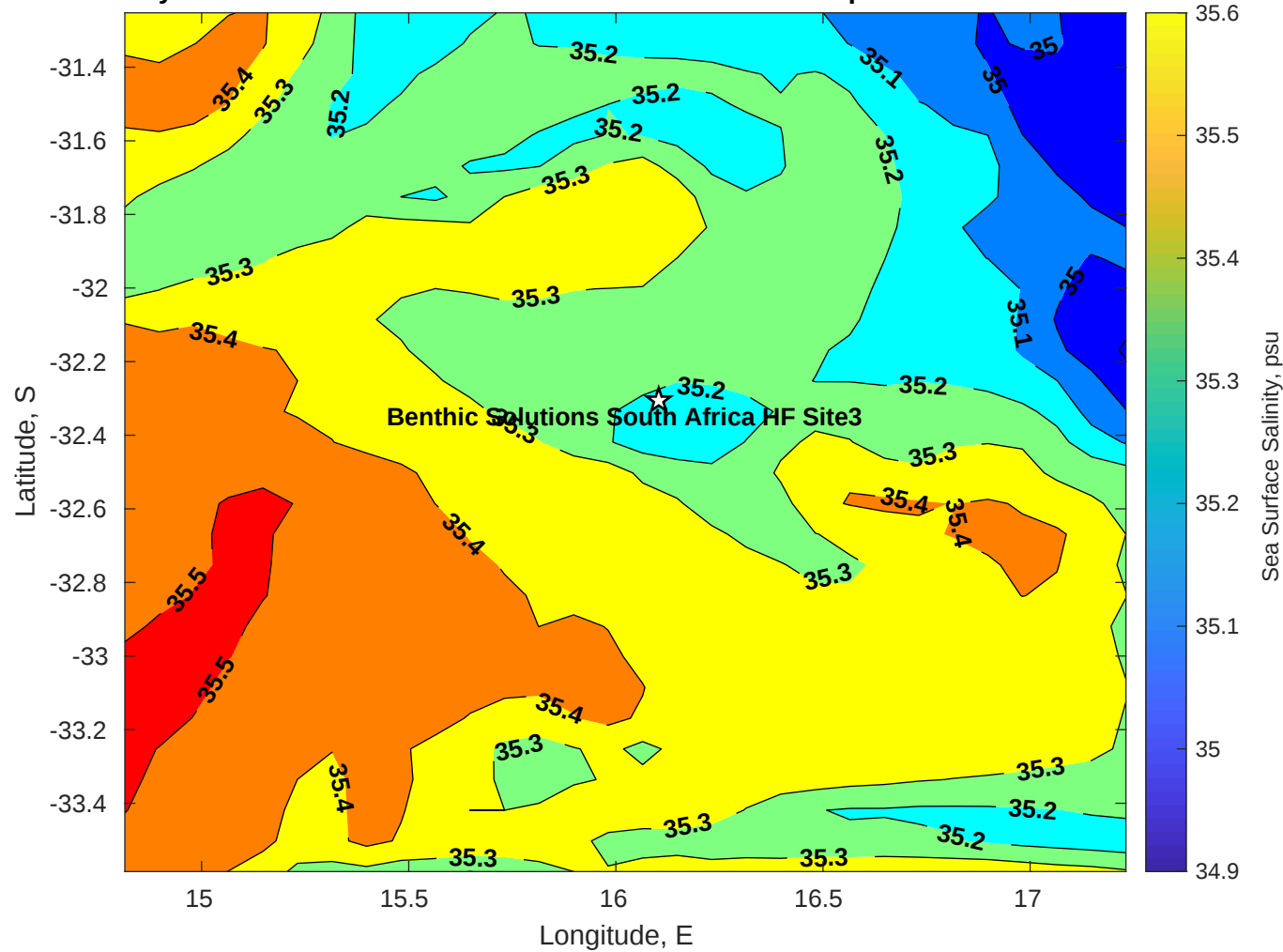
Surface Salinity for Benthic Solutions South Africa HF Site3 at 23-Apr-2025 00:00:00
