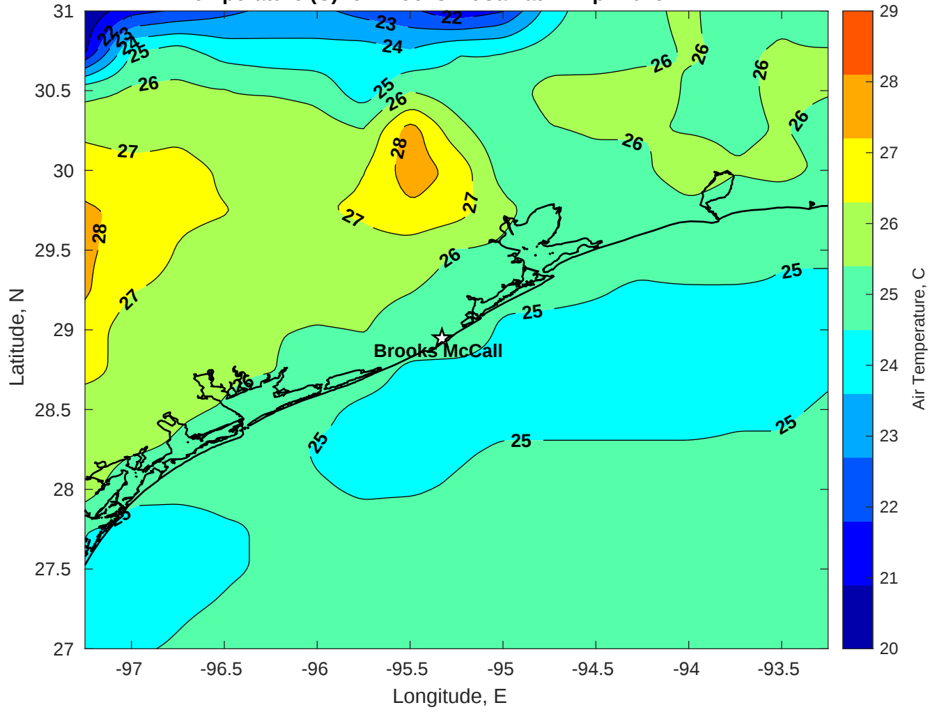
Air Temperature (C) for Brooks McCall at 24-Apr-2025
