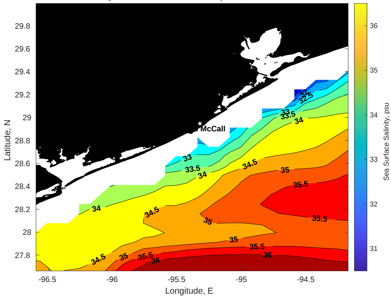
Surface Salinity for Brooks McCall at 23-Apr-2025 00:00:00
