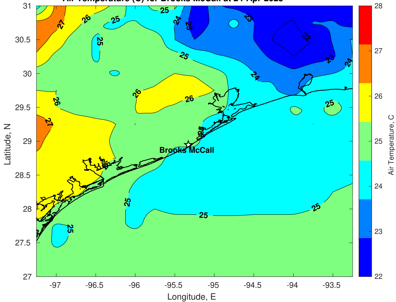
Air Temperature (C) for Brooks McCall at 24-Apr-2025
