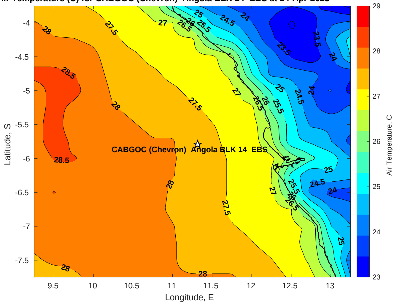
Air Temperature (C) for CABGOC (Chevron) Angola BLK 14 EBS at 24-Apr-2025
