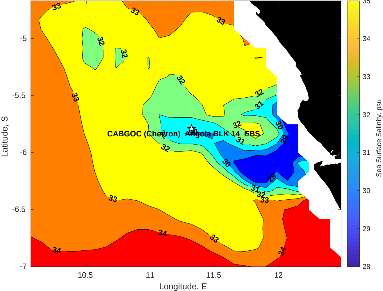
Surface Salinity for CABGOC (Chevron) Angola BLK 14 EBS at 23-Apr-2025 00:00:00
