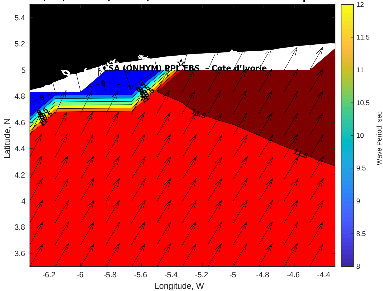
Wave Period (sec) for CSA (ONHYM) PPL EBS - Cote d'Ivoire at 24-Apr-2025 09:00:00
