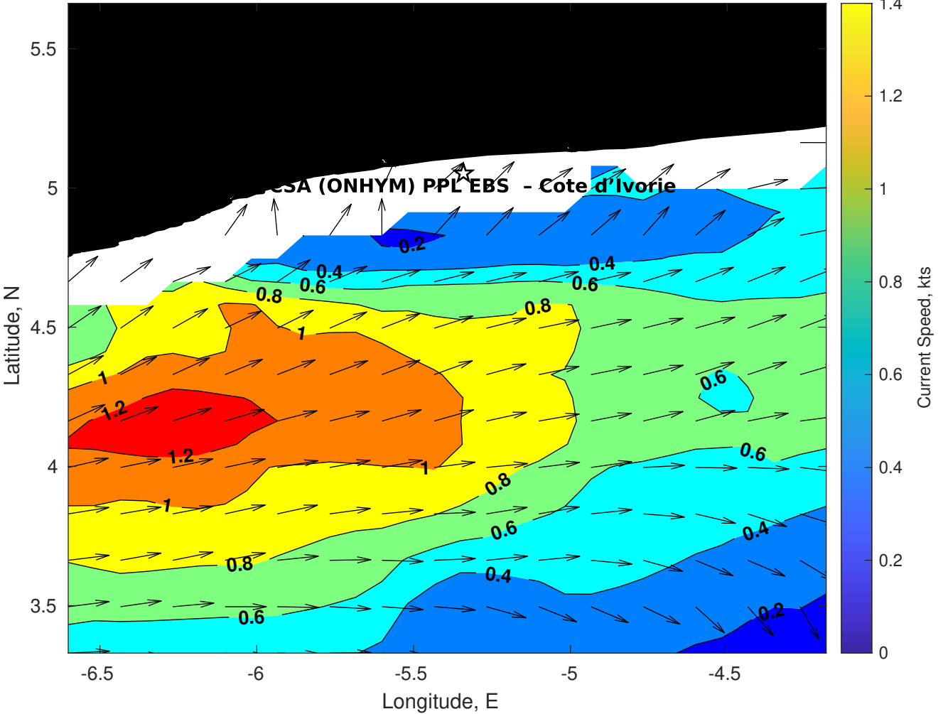
Surface Currents for CSA (ONHYM) PPL EBS - Cote d'Ivoire at 22-Apr-2025 00:00:00
