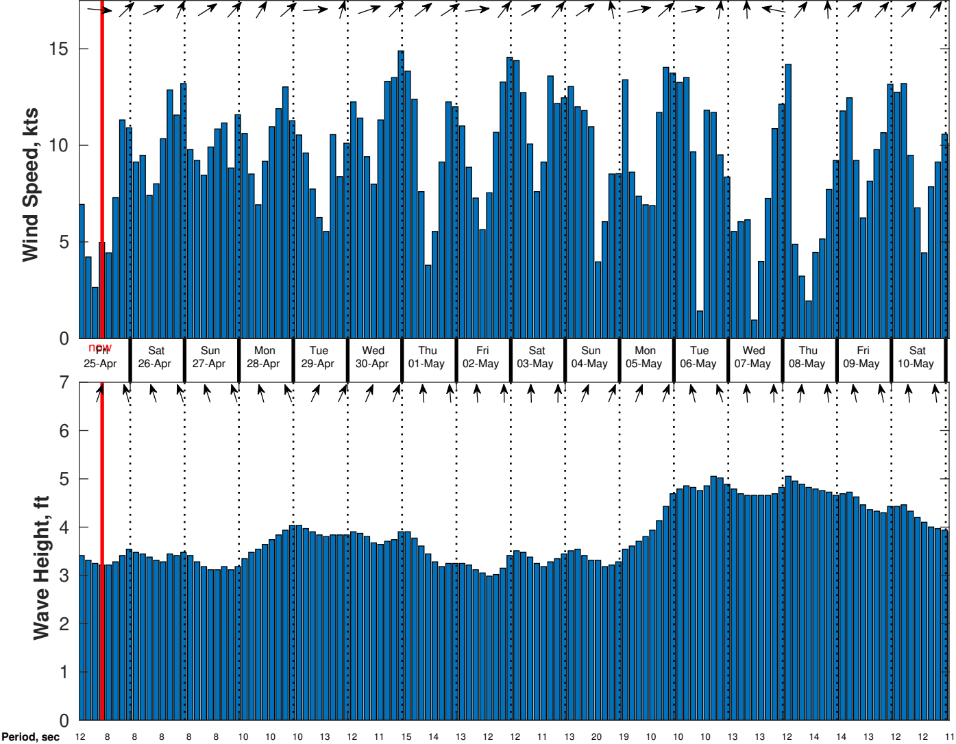
Wind & Wave Forecast for CSA (ONHYM) PPL EBS - Cote d'Ivoire from 24-Apr-2025 01:00:00 to 10-May-2025 01:00:00
