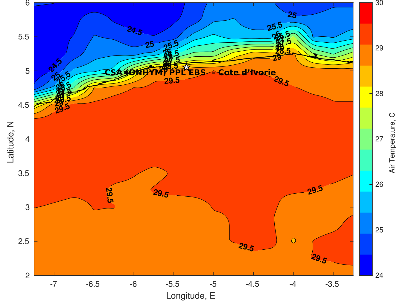
Air Temperature (C) for CSA (ONHYM) PPL EBS - Cote d'Ivoire at 24-Apr-2025
