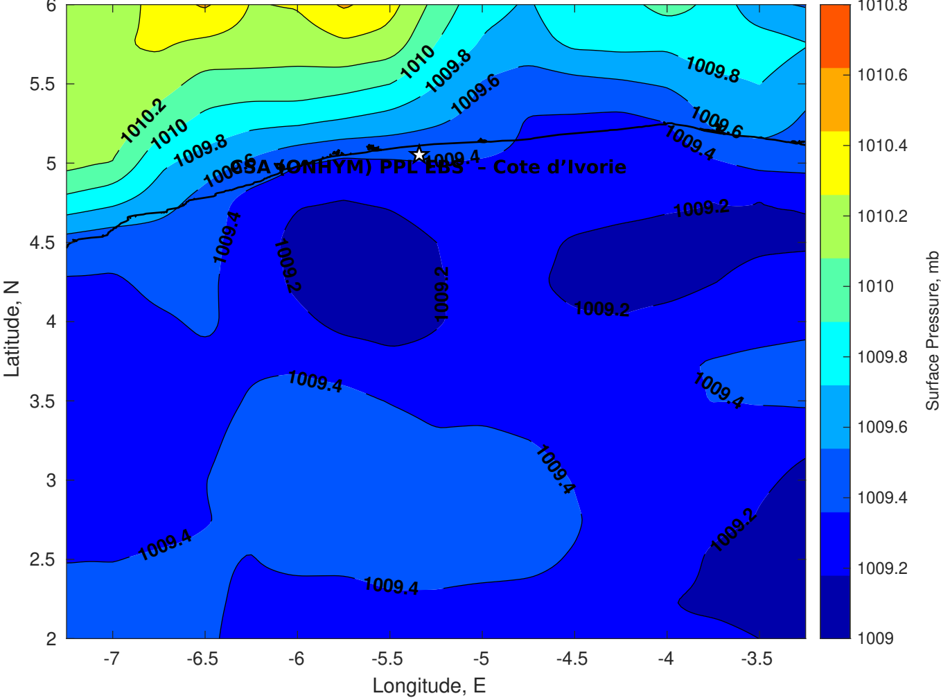
Surface Pressure (mb) for CSA (ONHYM) PPL EBS - Cote d'Ivoire at 26-Apr-2025 00:00:00
