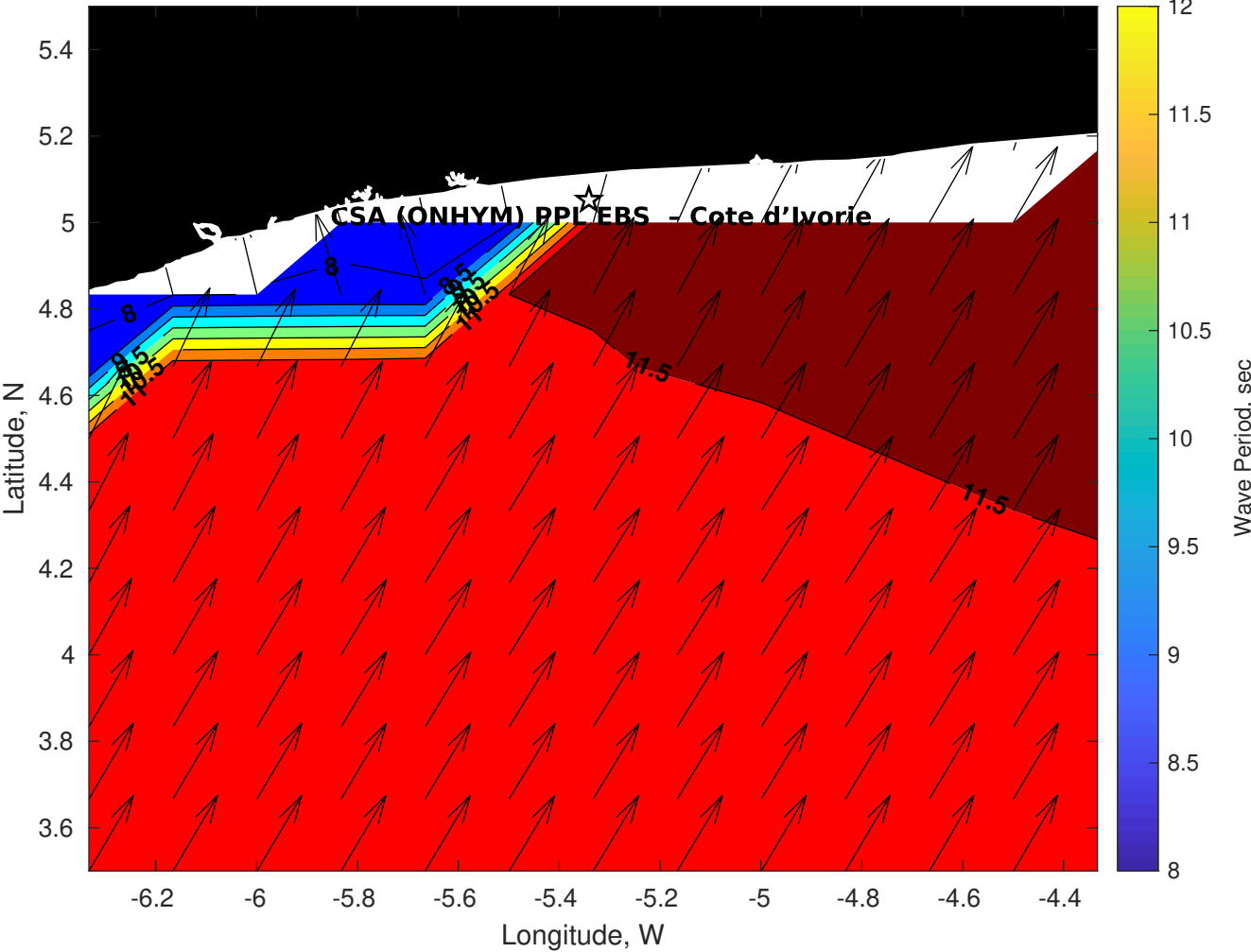
Wave Period (sec) for CSA (ONHYM) PPL EBS - Cote d'Ivoire at 24-Apr-2025 09:00:00
