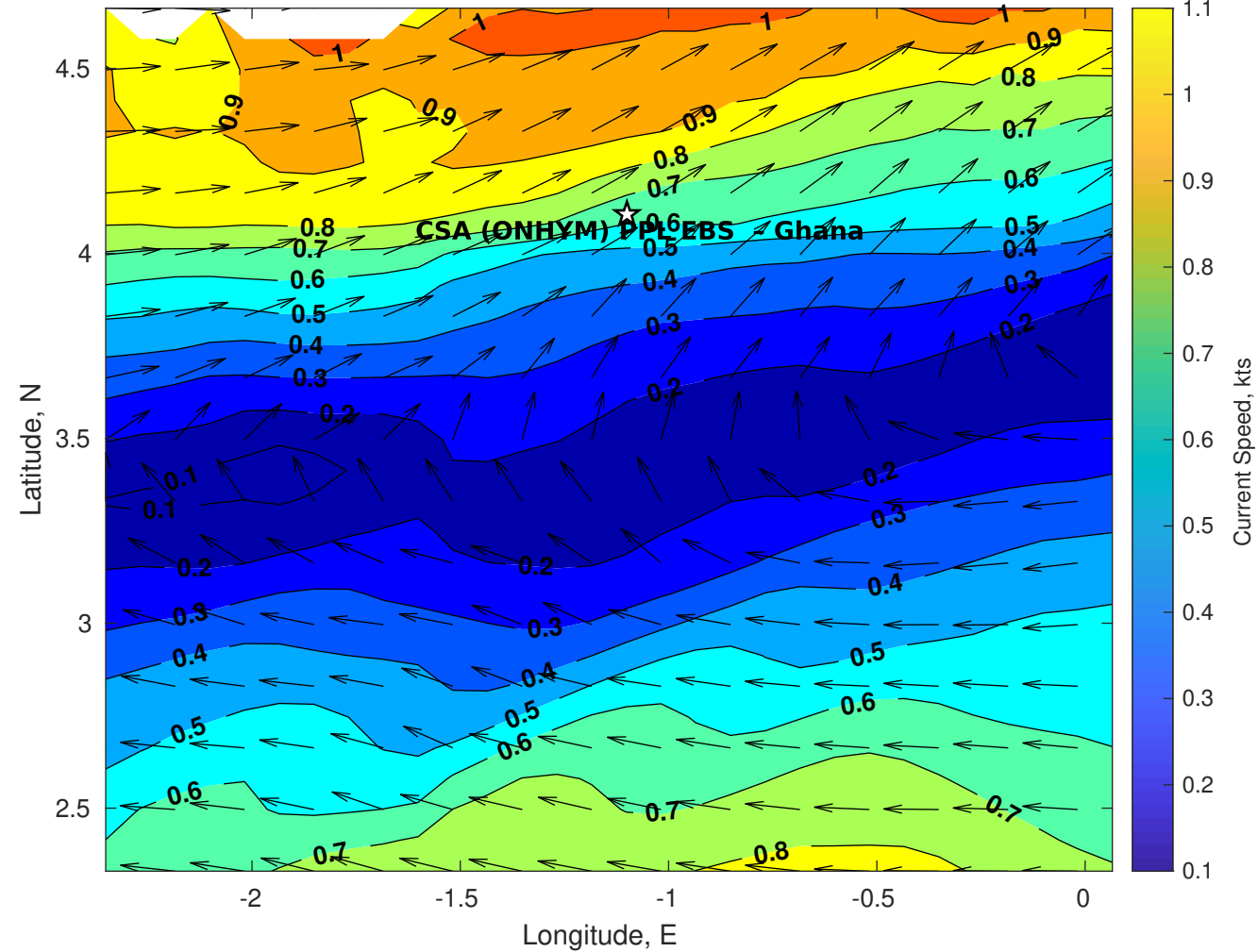
Surface Currents for CSA (ONHYM) PPL EBS - Ghana at 22-Apr-2025 00:00:00
