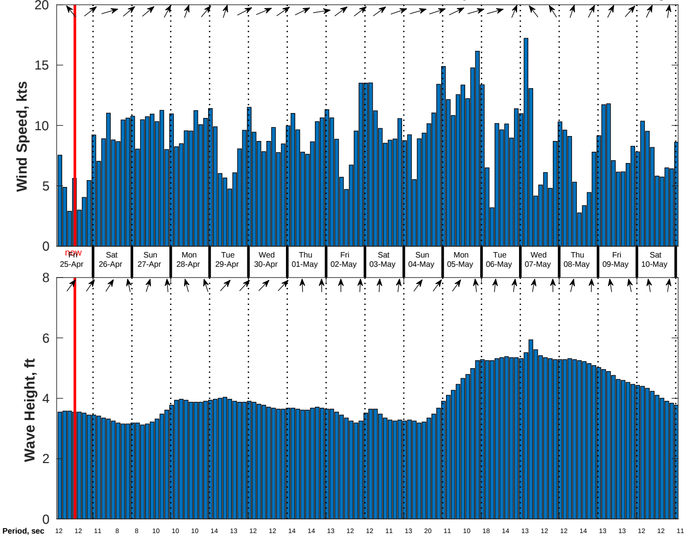
Wind & Wave Forecast for CSA (ONHYM) PPL EBS - Ghana from 24-Apr-2025 02:00:00 to 10-May-2025 02:00:00
