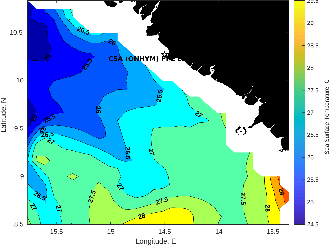
SST for CSA (ONHYM) PPL EBS - Guinea at 22-Apr-2025 00:00:00
