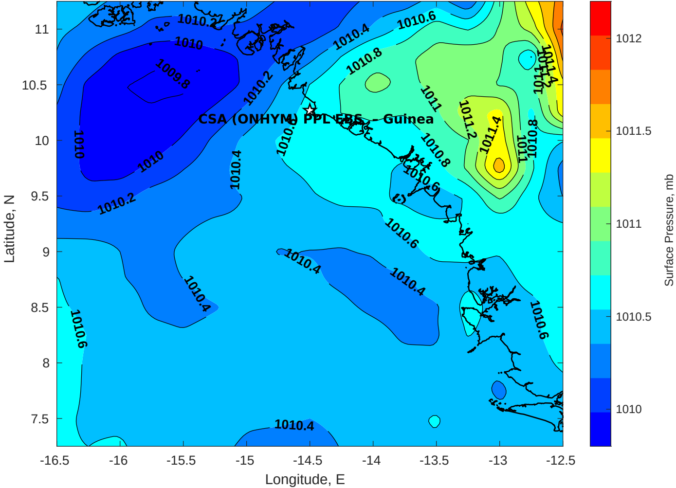
Surface Pressure (mb) for CSA (ONHYM) PPL EBS - Guinea at 25-Apr-2025 00:00:00
