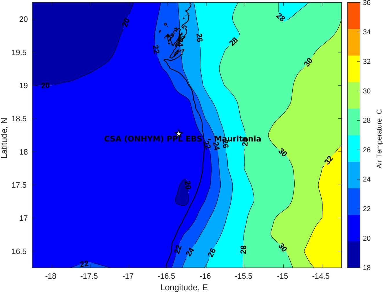
Air Temperature (C) for CSA (ONHYM) PPL EBS - Mauritania at 24-Apr-2025
