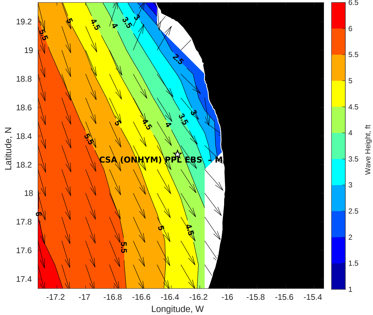
Wave Height (ft) for CSA (ONHYM) PPL EBS - Mauritania at 24-Apr-2025 09:00:00
