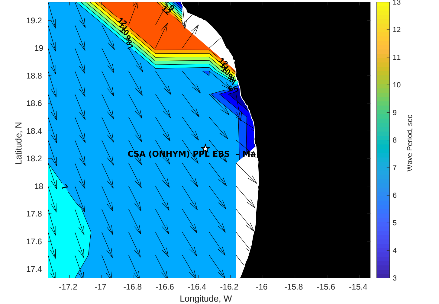
Wave Period (sec) for CSA (ONHYM) PPL EBS - Mauritania at 24-Apr-2025 09:00:00
