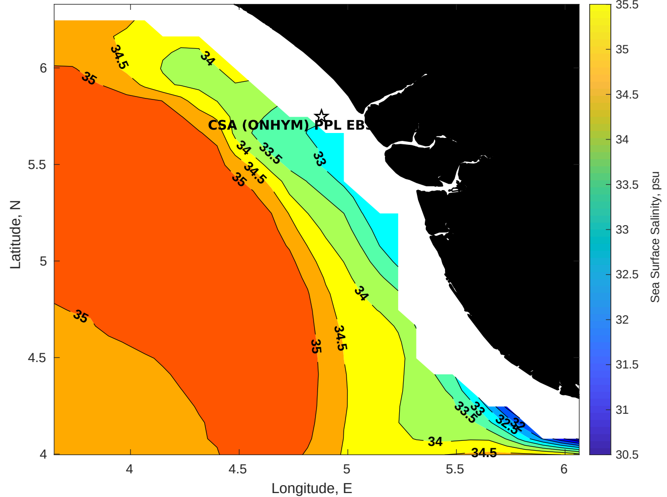
Surface Salinity for CSA (ONHYM) PPL EBS - Nigeria at 22-Apr-2025 00:00:00
