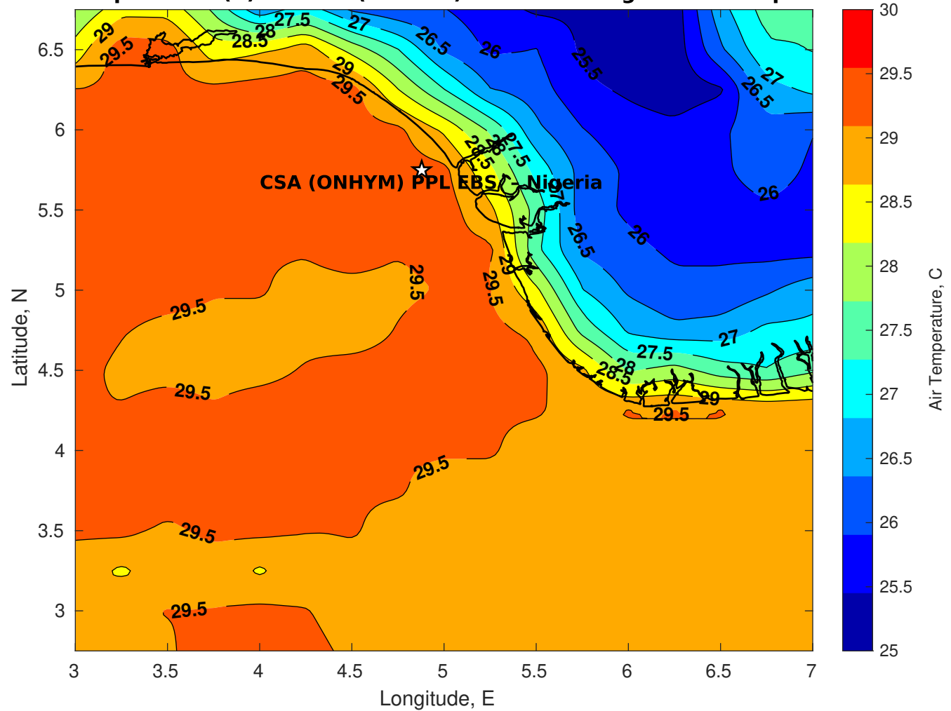
Air Temperature (C) for CSA (ONHYM) PPL EBS - Nigeria at 24-Apr-2025
