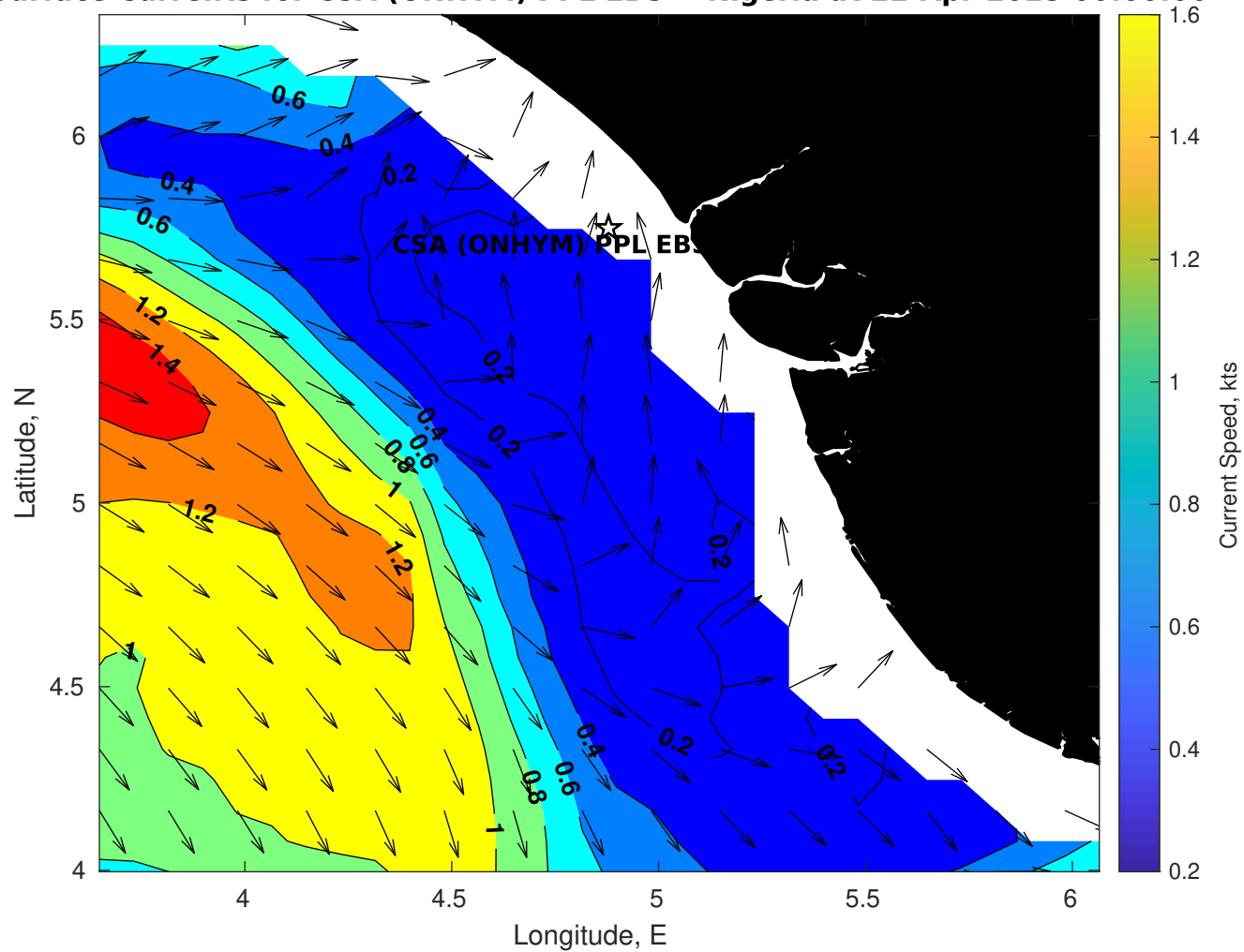
Surface Currents for CSA (ONHYM) PPL EBS - Nigeria at 22-Apr-2025 00:00:00
