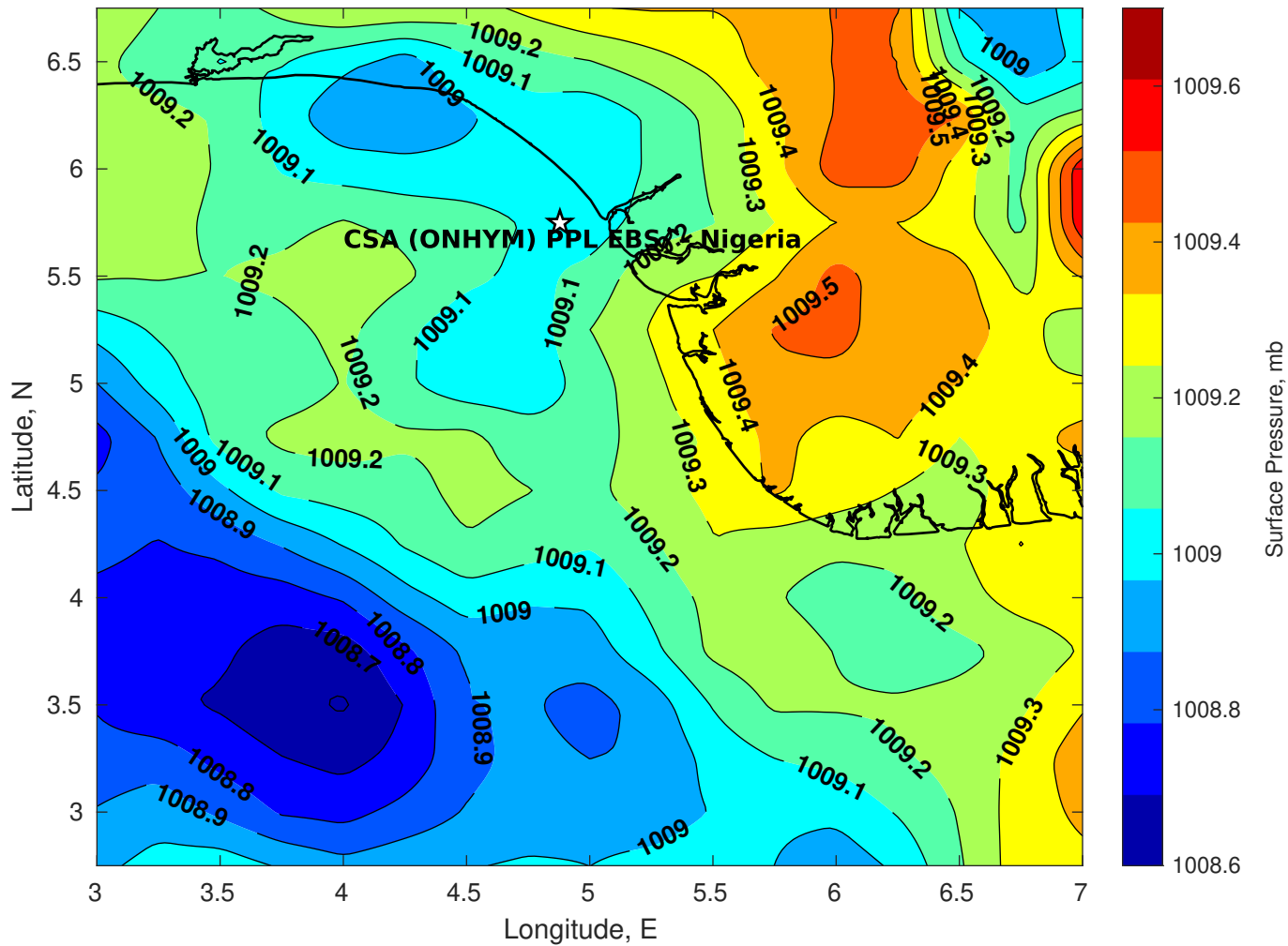
Surface Pressure (mb) for CSA (ONHYM) PPL EBS - Nigeria at 24-Apr-2025 00:00:00
