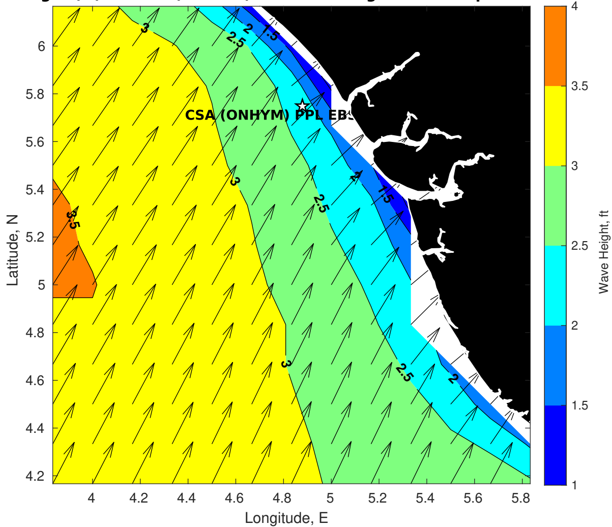
Wave Height (ft) for CSA (ONHYM) PPL EBS - Nigeria at 24-Apr-2025 09:00:00
