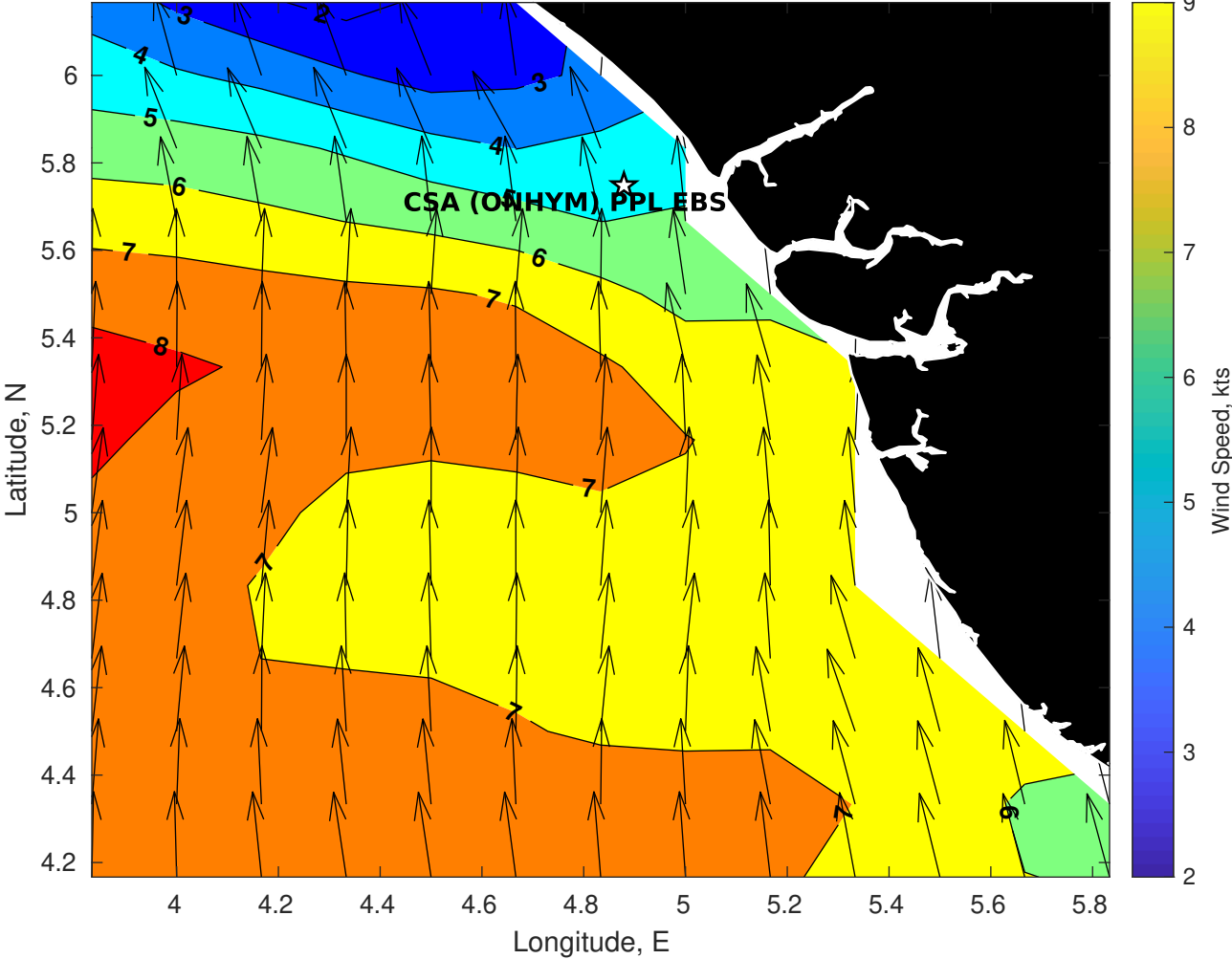
Winds (kts) for CSA (ONHYM) PPL EBS - Nigeria at 24-Apr-2025 09:00:00
