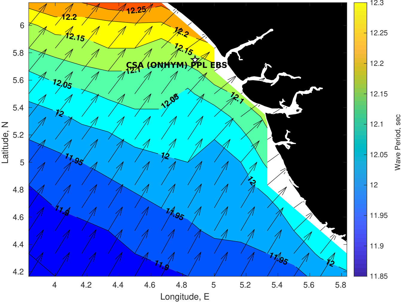
Wave Period (sec) for CSA (ONHYM) PPL EBS - Nigeria at 24-Apr-2025 09:00:00
