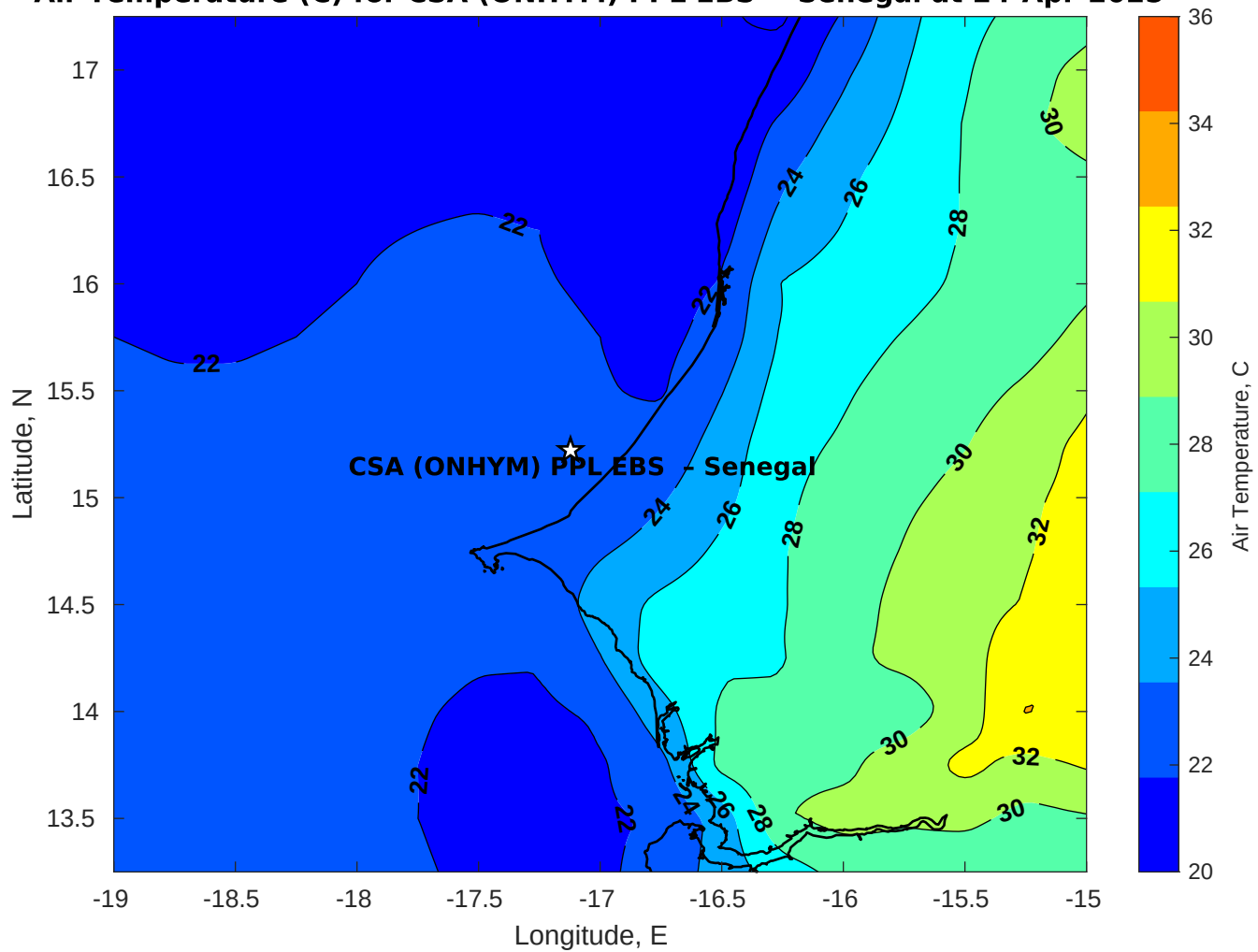
Air Temperature (C) for CSA (ONHYM) PPL EBS - Senegal at 24-Apr-2025
