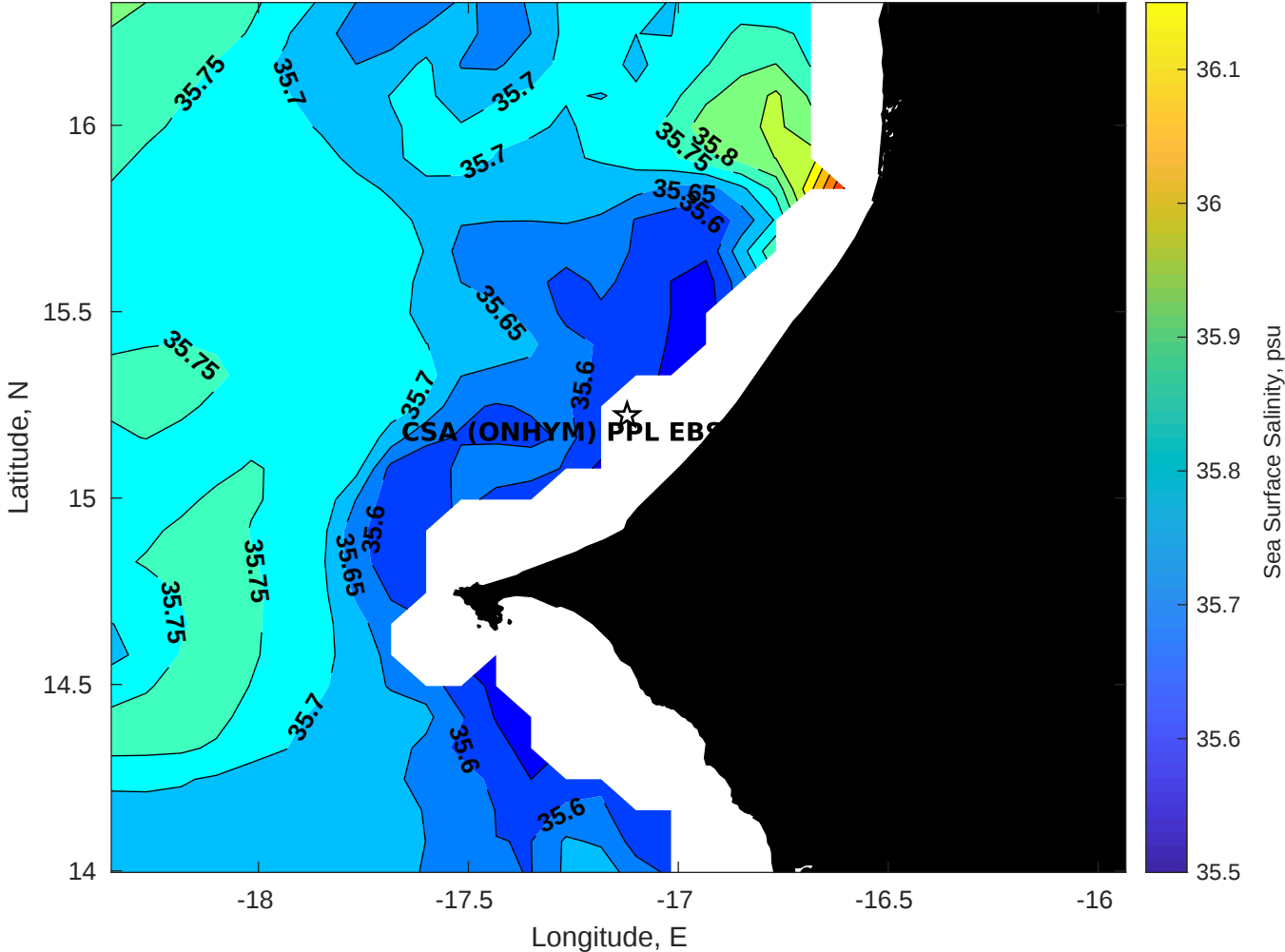
Surface Salinity for CSA (ONHYM) PPL EBS - Senegal at 22-Apr-2025 00:00:00
