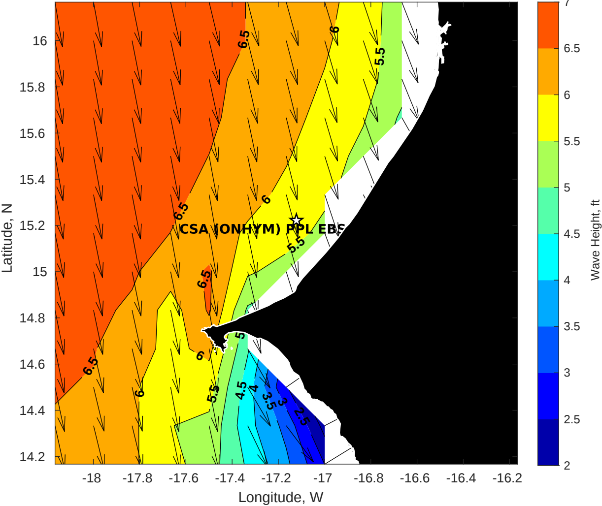
Wave Height (ft) for CSA (ONHYM) PPL EBS - Senegal at 24-Apr-2025 09:00:00
