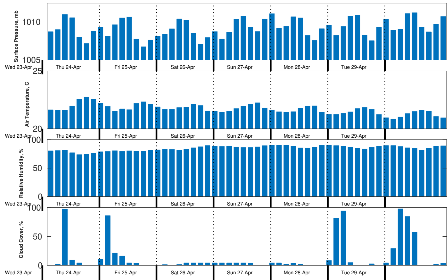
Met Forecast for CSA (ONHYM) PPL EBS - Senegal from 24-Apr-2025 00:00:00 to 01-May-2025 00:00:00
