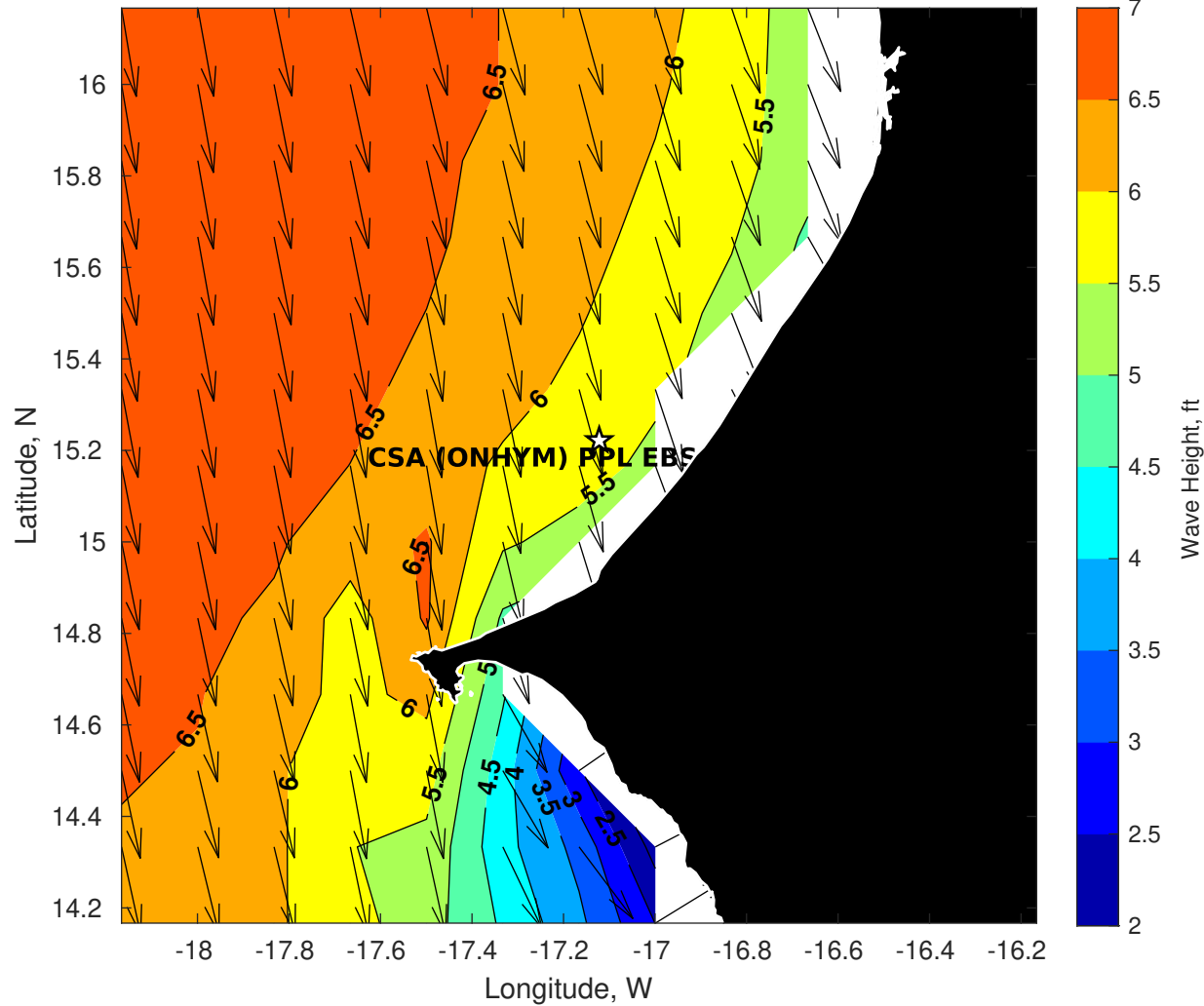
Wave Height (ft) for CSA (ONHYM) PPL EBS - Senegal at 24-Apr-2025 09:00:00
