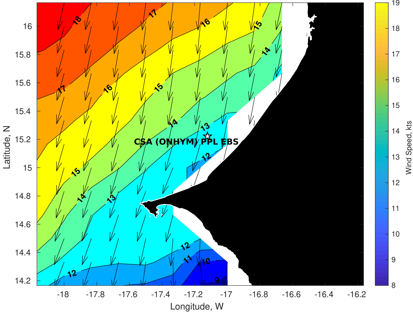
Winds (kts) for CSA (ONHYM) PPL EBS - Senegal at 24-Apr-2025 09:00:00
