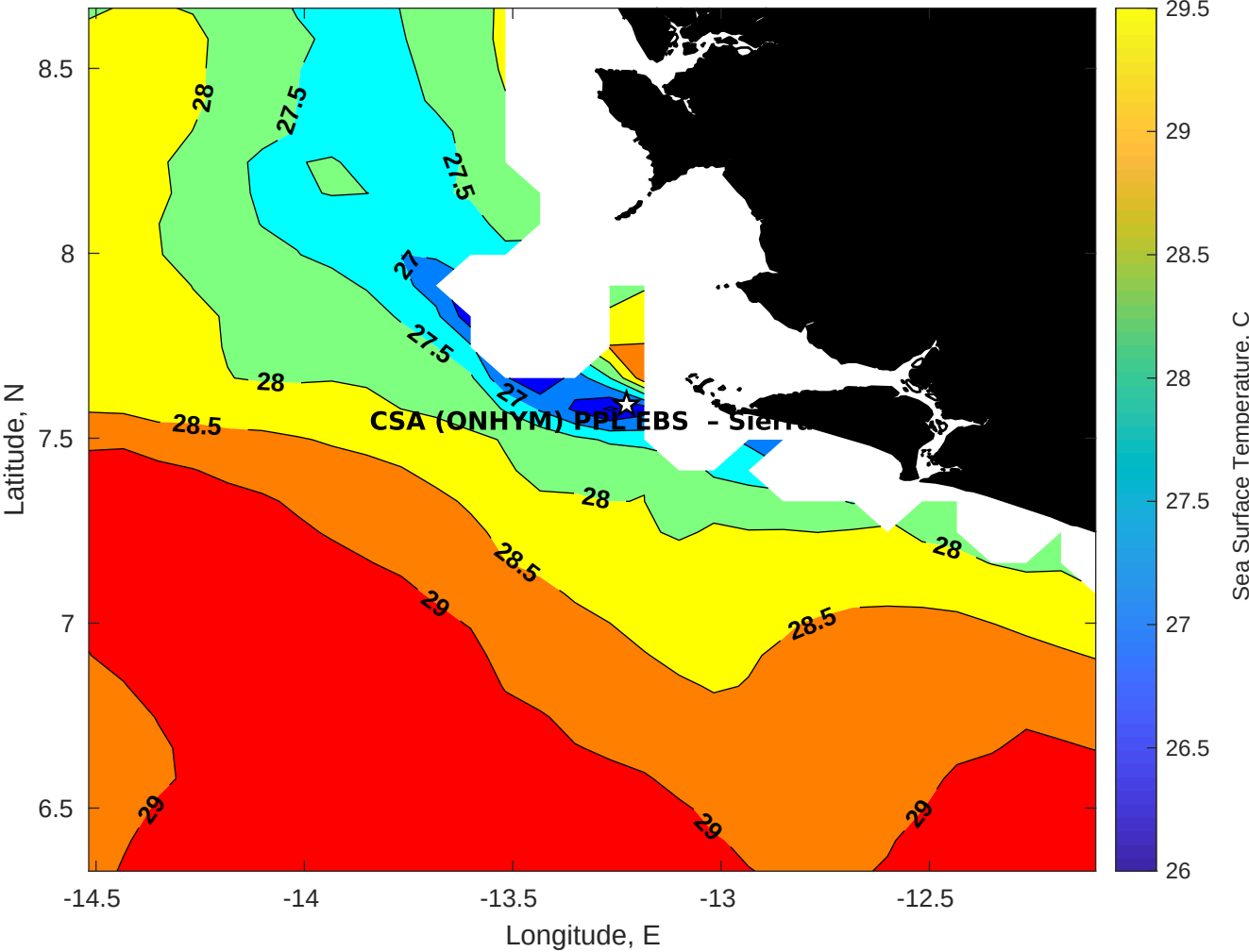
SST for CSA (ONHYM) PPL EBS - Sierra Leone at 22-Apr-2025 00:00:00
