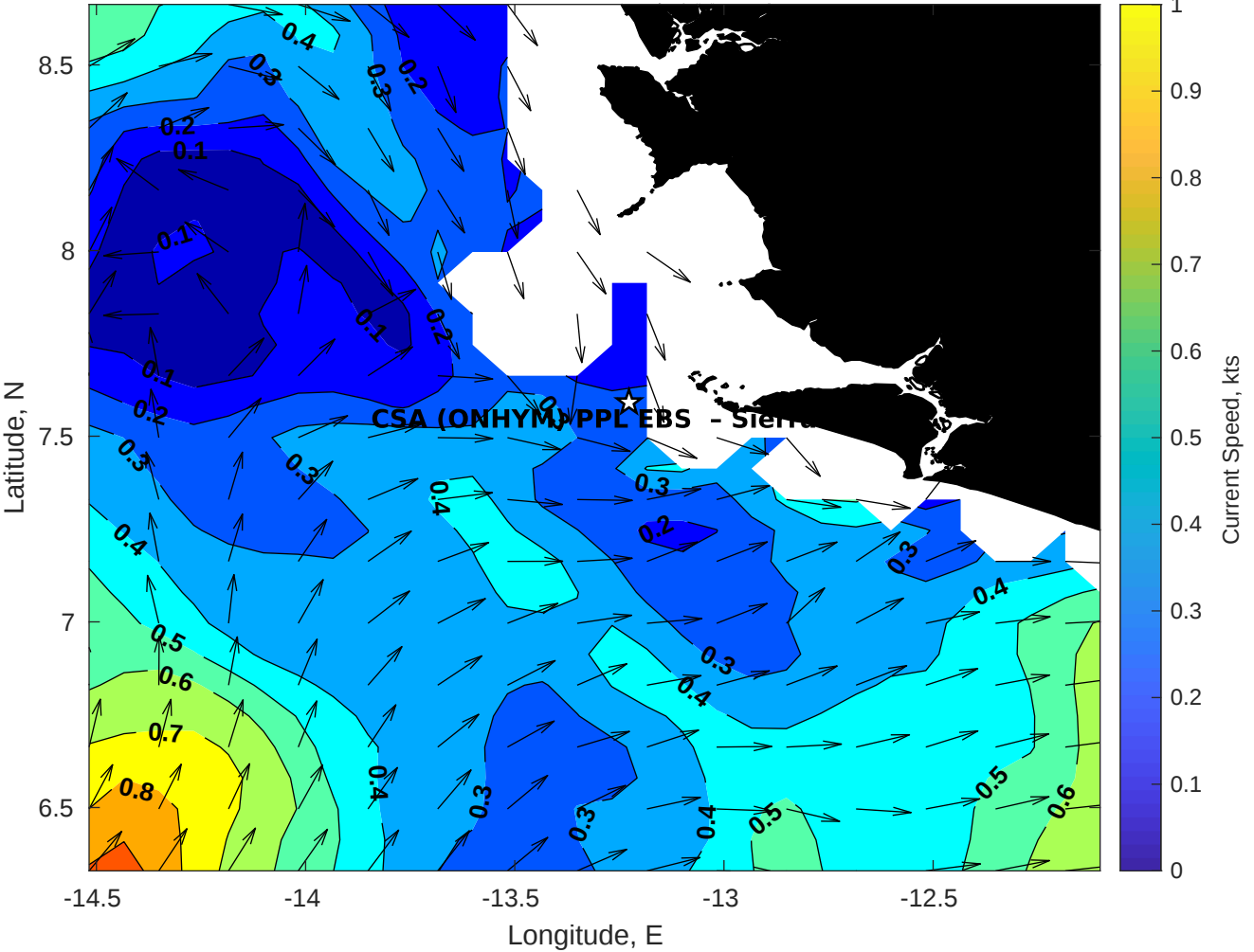
Surface Currents for CSA (ONHYM) PPL EBS - Sierra Leone at 22-Apr-2025 00:00:00
