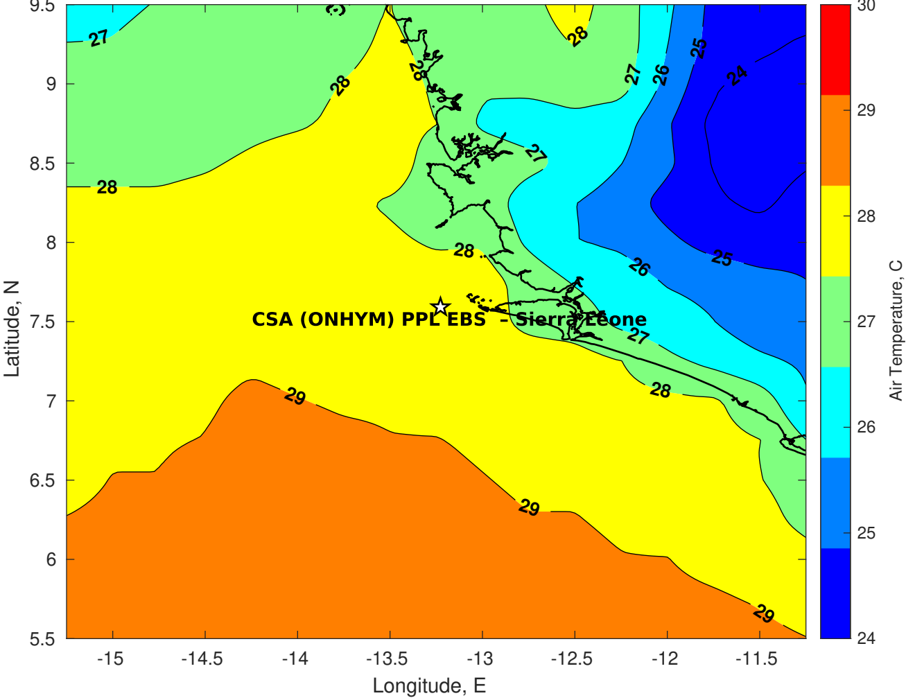
Air Temperature (C) for CSA (ONHYM) PPL EBS - Sierra Leone at 24-Apr-2025
