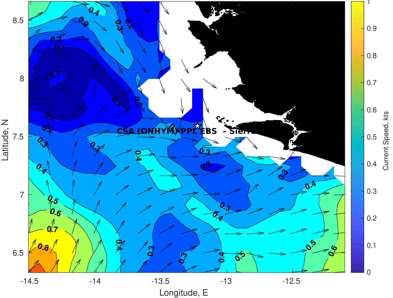
Surface Currents for CSA (ONHYM) PPL EBS - Sierra Leone at 22-Apr-2025 00:00:00
