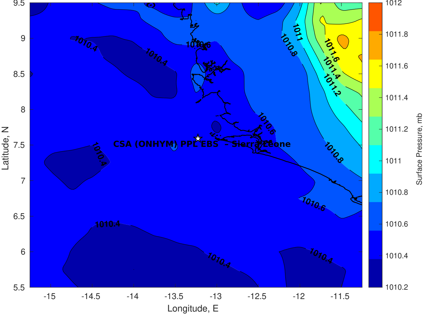
Surface Pressure (mb) for CSA (ONHYM) PPL EBS - Sierra Leone at 25-Apr-2025 00:00:00
