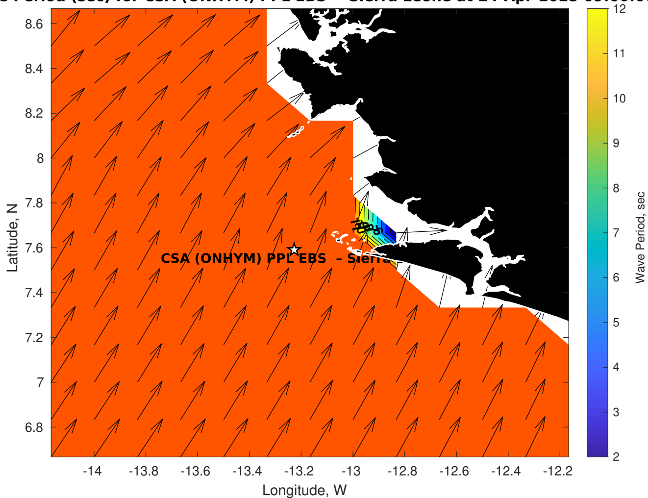
Wave Period (sec) for CSA (ONHYM) PPL EBS - Sierra Leone at 24-Apr-2025 09:00:00
