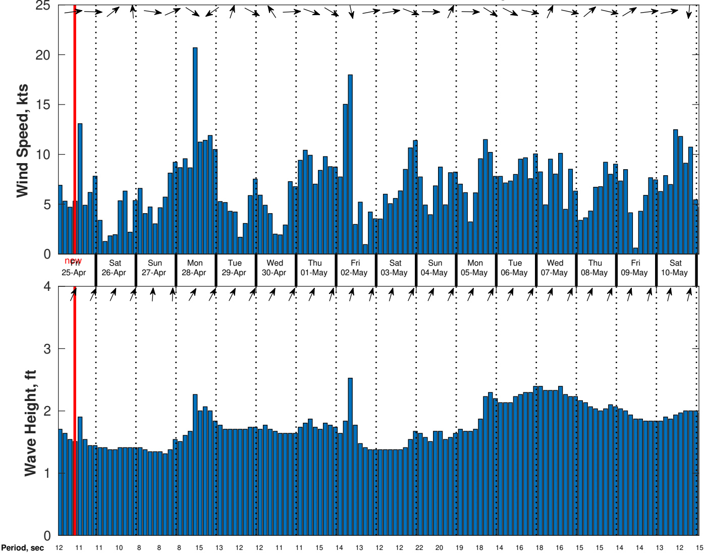
Wind & Wave Forecast for CSA (ONHYM) PPL EBS - Sierra Leone from 24-Apr-2025 01:00:00 to 10-May-2025 01:00:00
