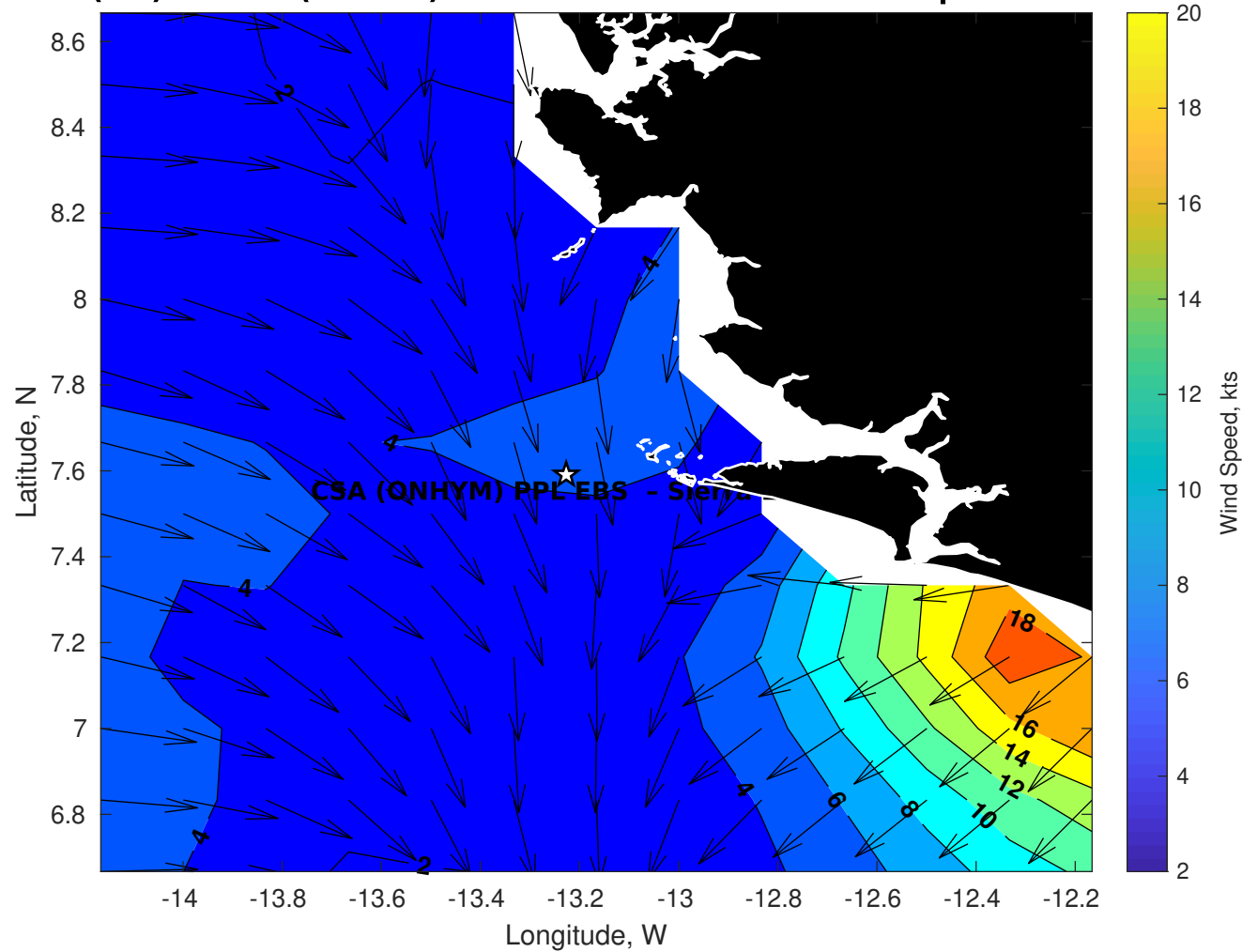
Winds (kts) for CSA (ONHYM) PPL EBS - Sierra Leone at 24-Apr-2025 09:00:00
