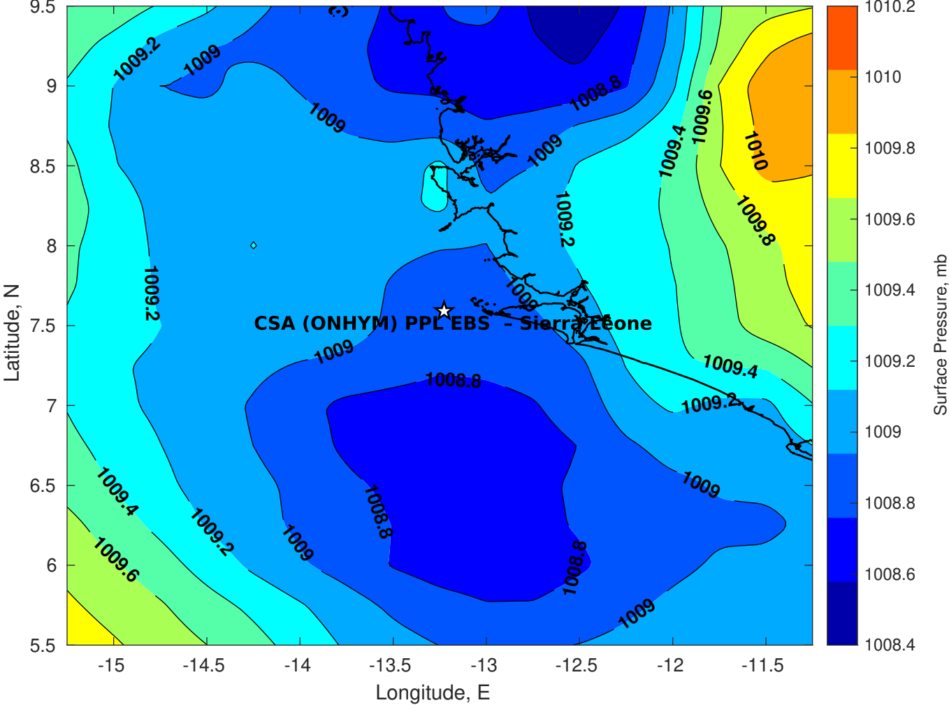
Surface Pressure (mb) for CSA (ONHYM) PPL EBS - Sierra Leone at 26-Apr-2025 00:00:00
