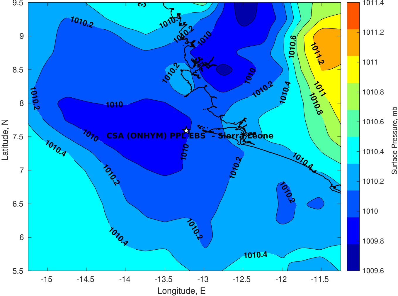
Surface Pressure (mb) for CSA (ONHYM) PPL EBS - Sierra Leone at 24-Apr-2025 00:00:00
