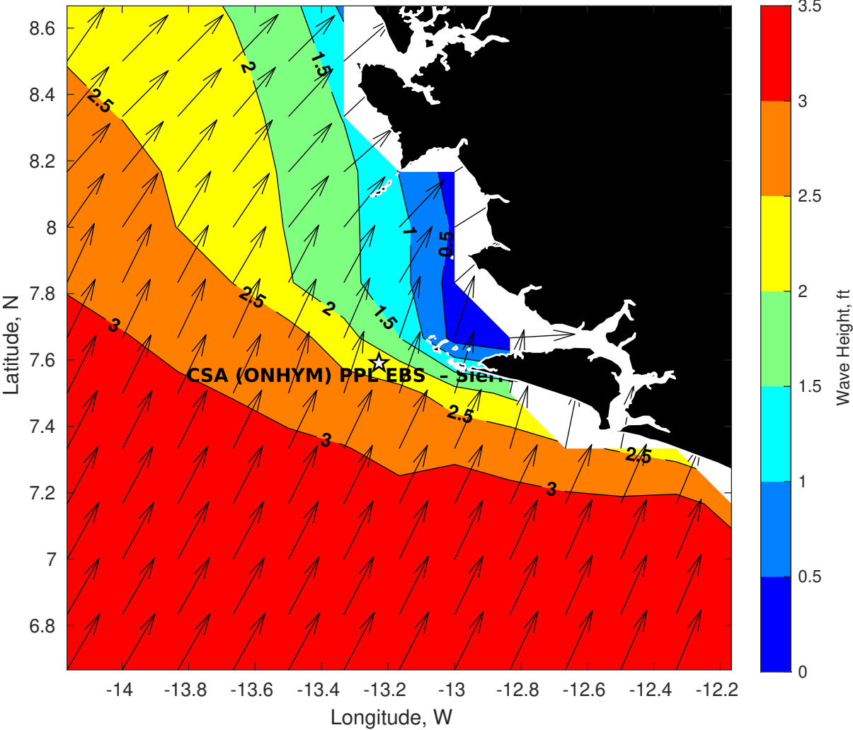
Wave Height (ft) for CSA (ONHYM) PPL EBS - Sierra Leone at 24-Apr-2025 09:00:00
