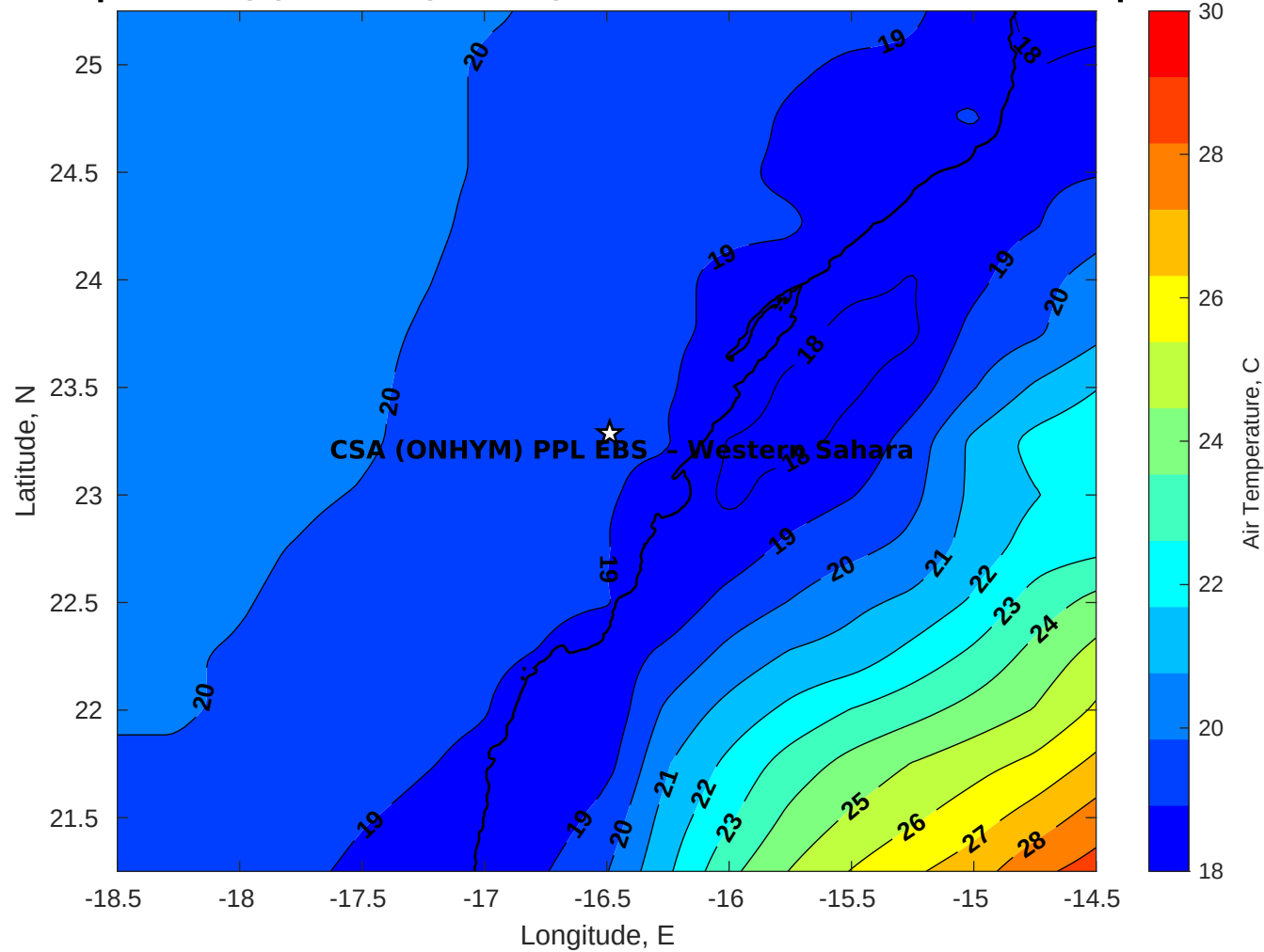
Air Temperature (C) for CSA (ONHYM) PPL EBS - Western Sahara at 24-Apr-2025
