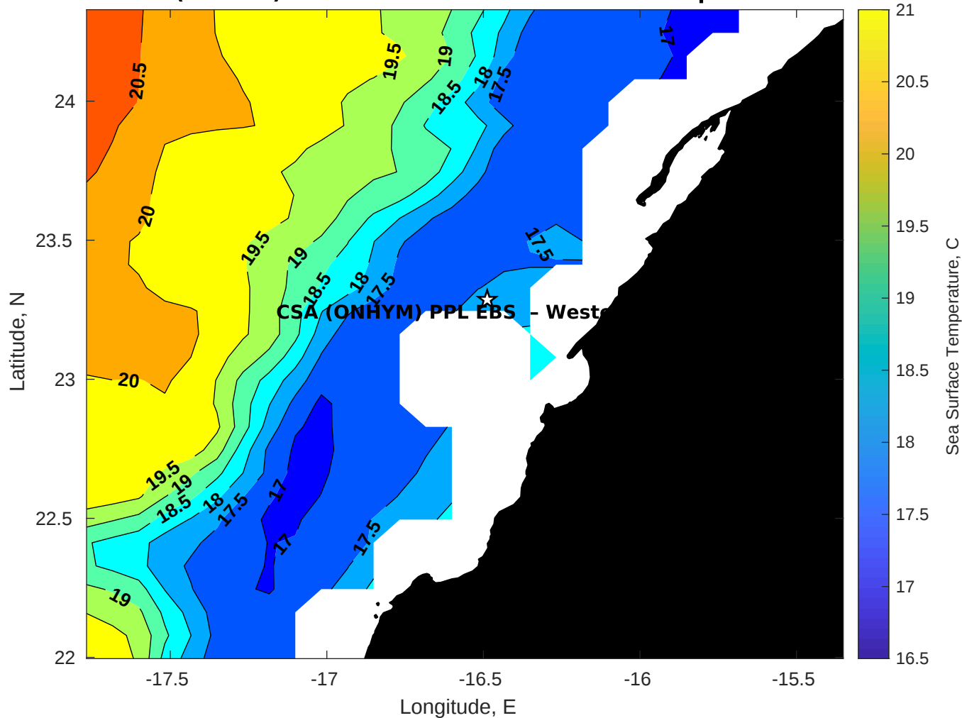
SST for CSA (ONHYM) PPL EBS - Western Sahara at 23-Apr-2025 00:00:00
