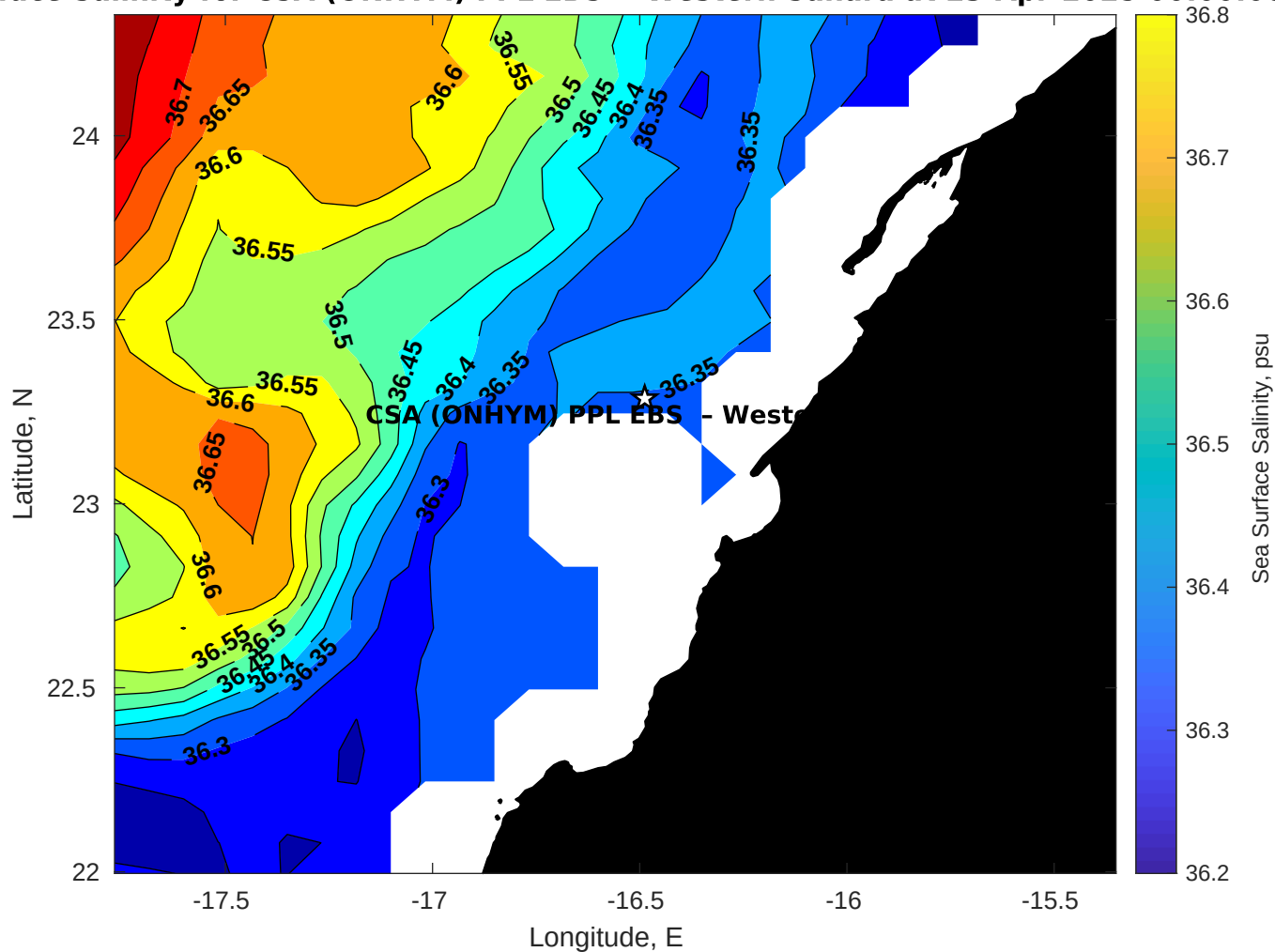
Surface Salinity for CSA (ONHYM) PPL EBS - Western Sahara at 23-Apr-2025 00:00:00
