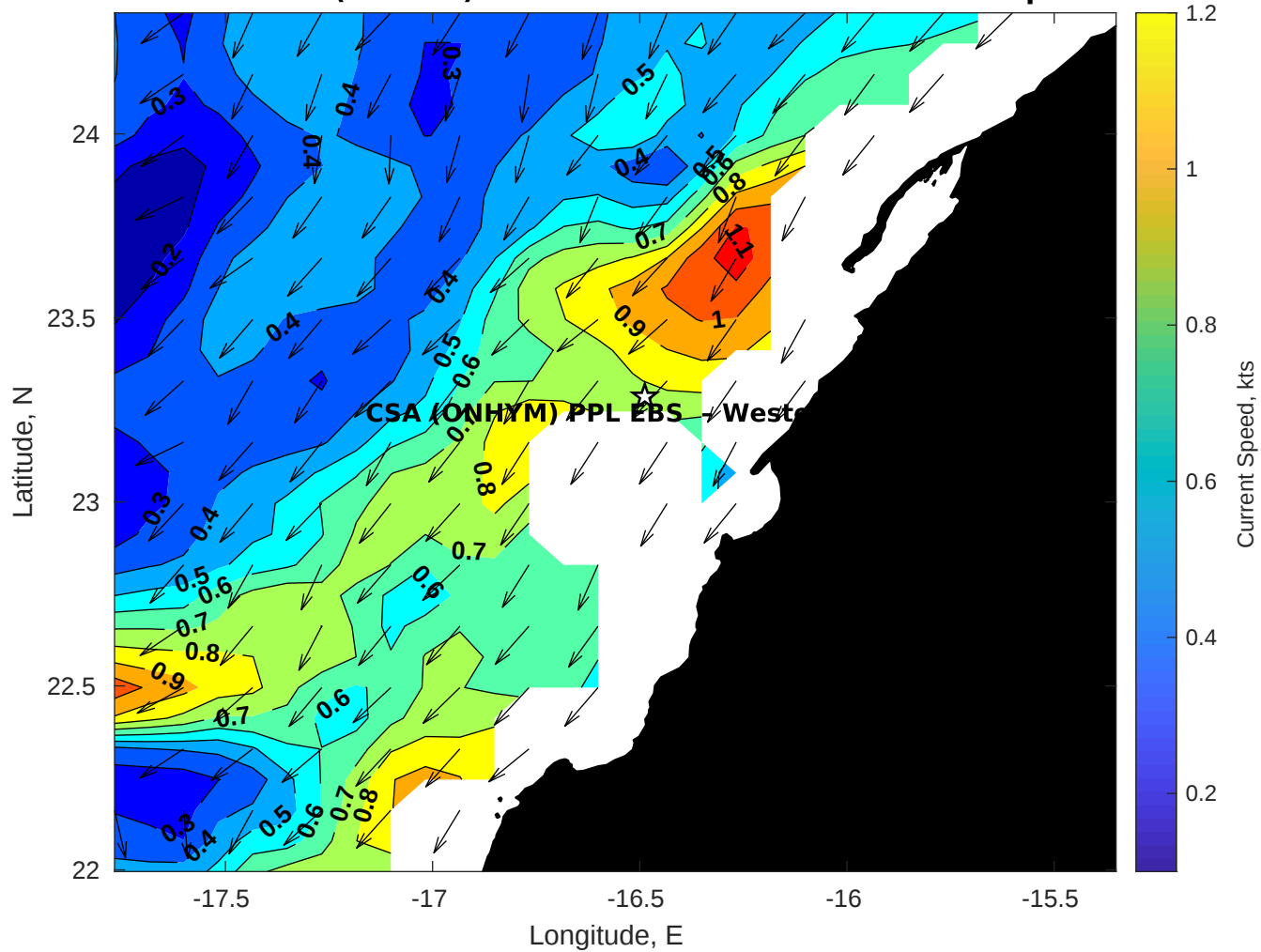
Surface Currents for CSA (ONHYM) PPL EBS - Western Sahara at 23-Apr-2025 00:00:00
