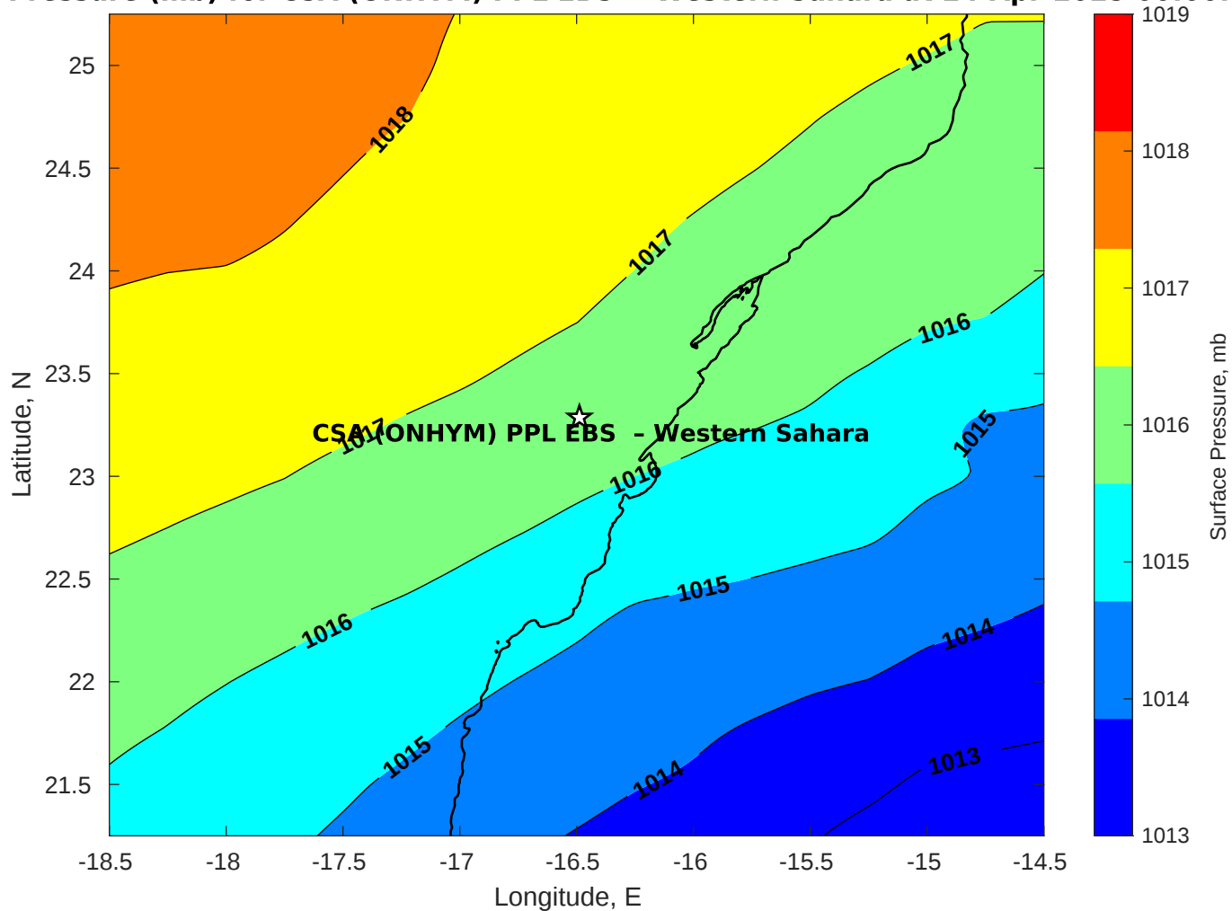
Surface Pressure (mb) for CSA (ONHYM) PPL EBS - Western Sahara at 24-Apr-2025 00:00:00
