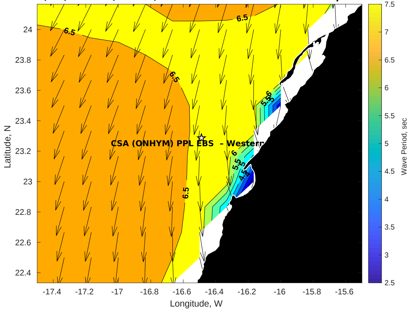
Wave Period (sec) for CSA (ONHYM) PPL EBS - Western Sahara at 24-Apr-2025 09:00:00
