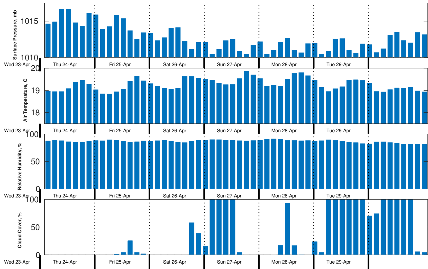
Met Forecast for CSA (ONHYM) PPL EBS - Western Sahara from 24-Apr-2025 00:00:00 to 01-May-2025 00:00:00
