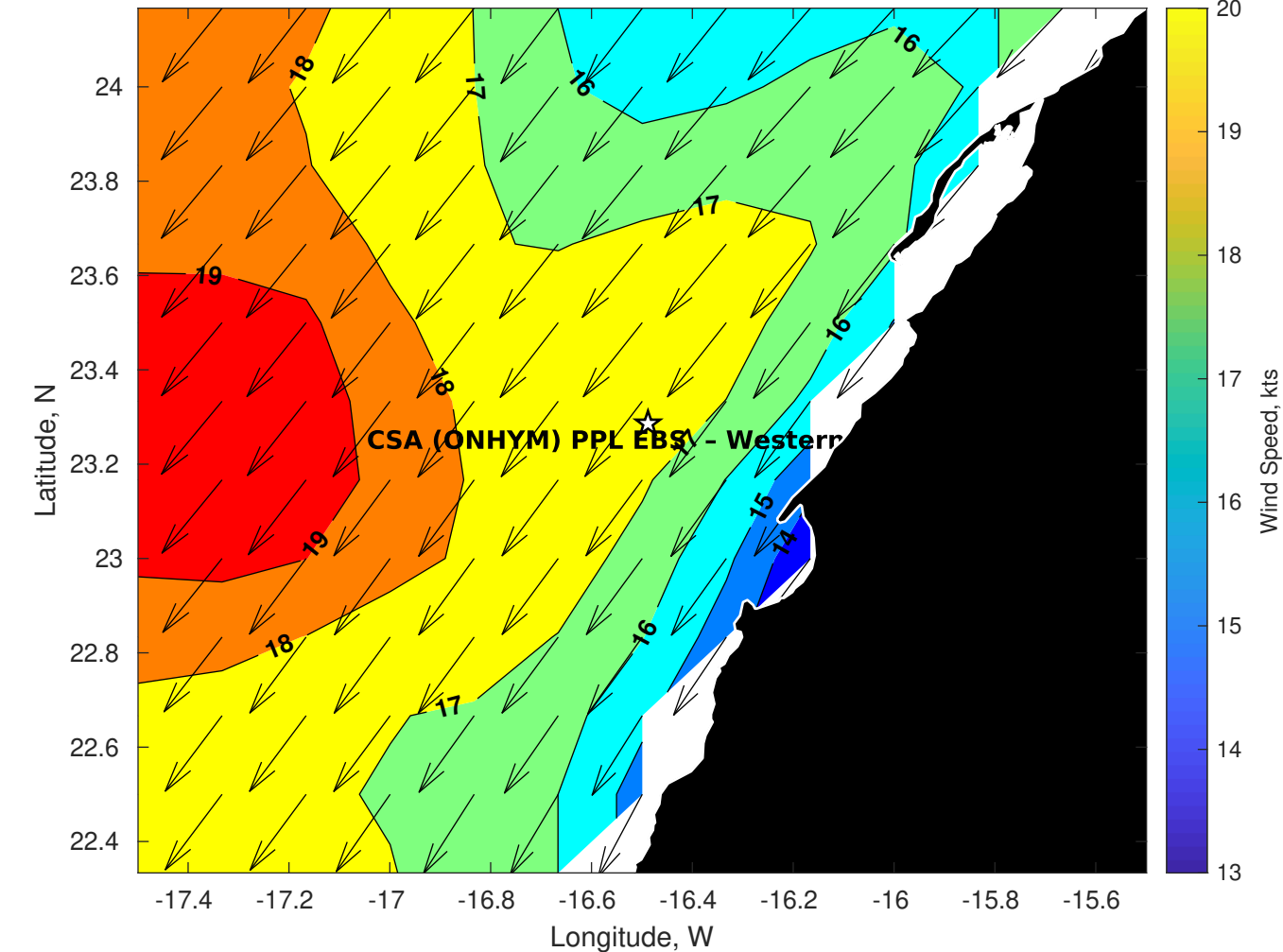
Winds (kts) for CSA (ONHYM) PPL EBS - Western Sahara at 24-Apr-2025 09:00:00
