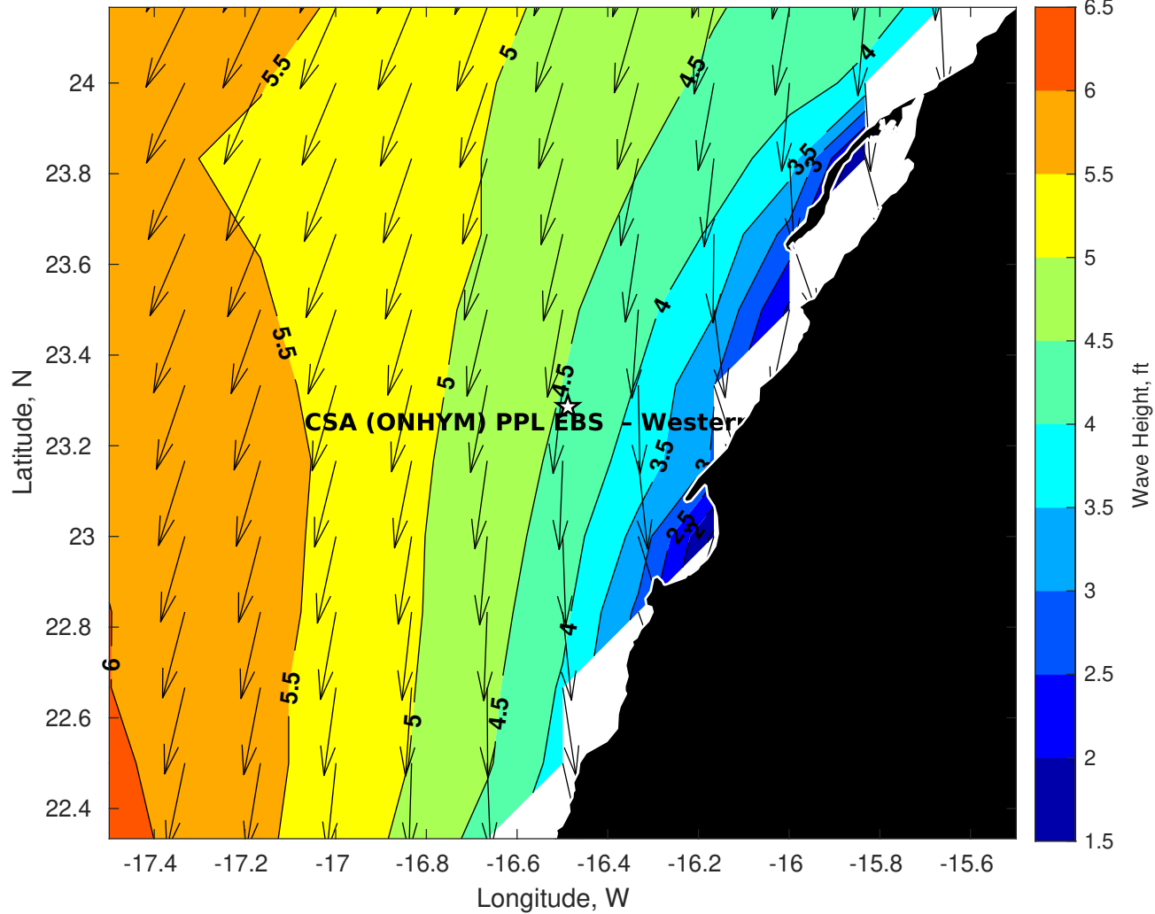
Wave Height (ft) for CSA (ONHYM) PPL EBS - Western Sahara at 24-Apr-2025 09:00:00
