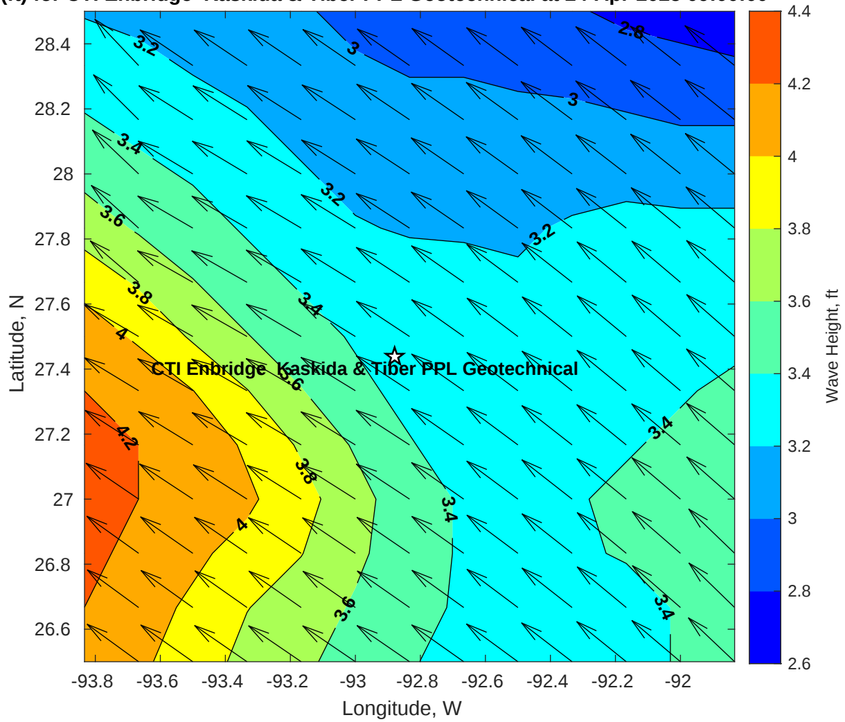
Wave Height (ft) for CTI Enbridge Kaskida & Tiber PPL Geotechnical at 24-Apr-2025 09:00:00
