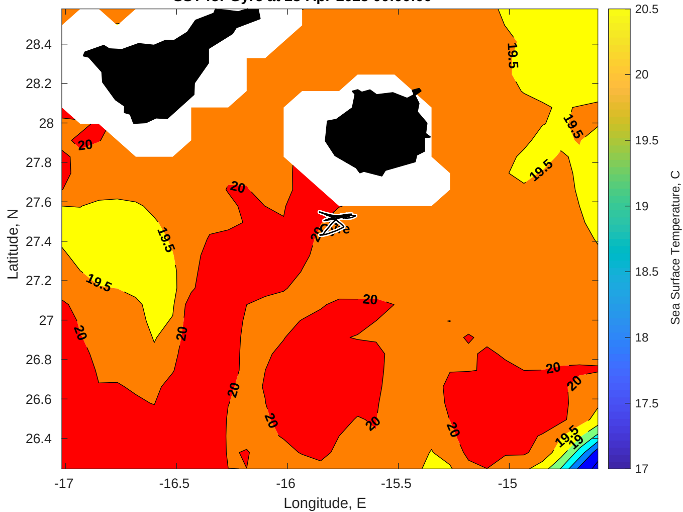
SST for Gyre at 23-Apr-2025 00:00:00
