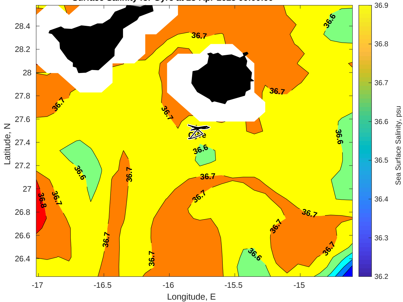
Surface Salinity for Gyre at 23-Apr-2025 00:00:00
