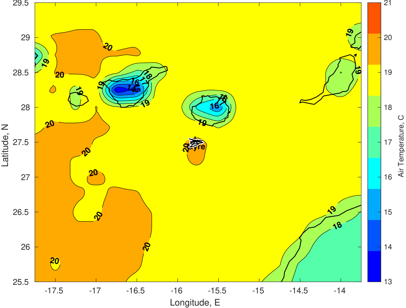
Air Temperature (C) for Gyre at 24-Apr-2025
