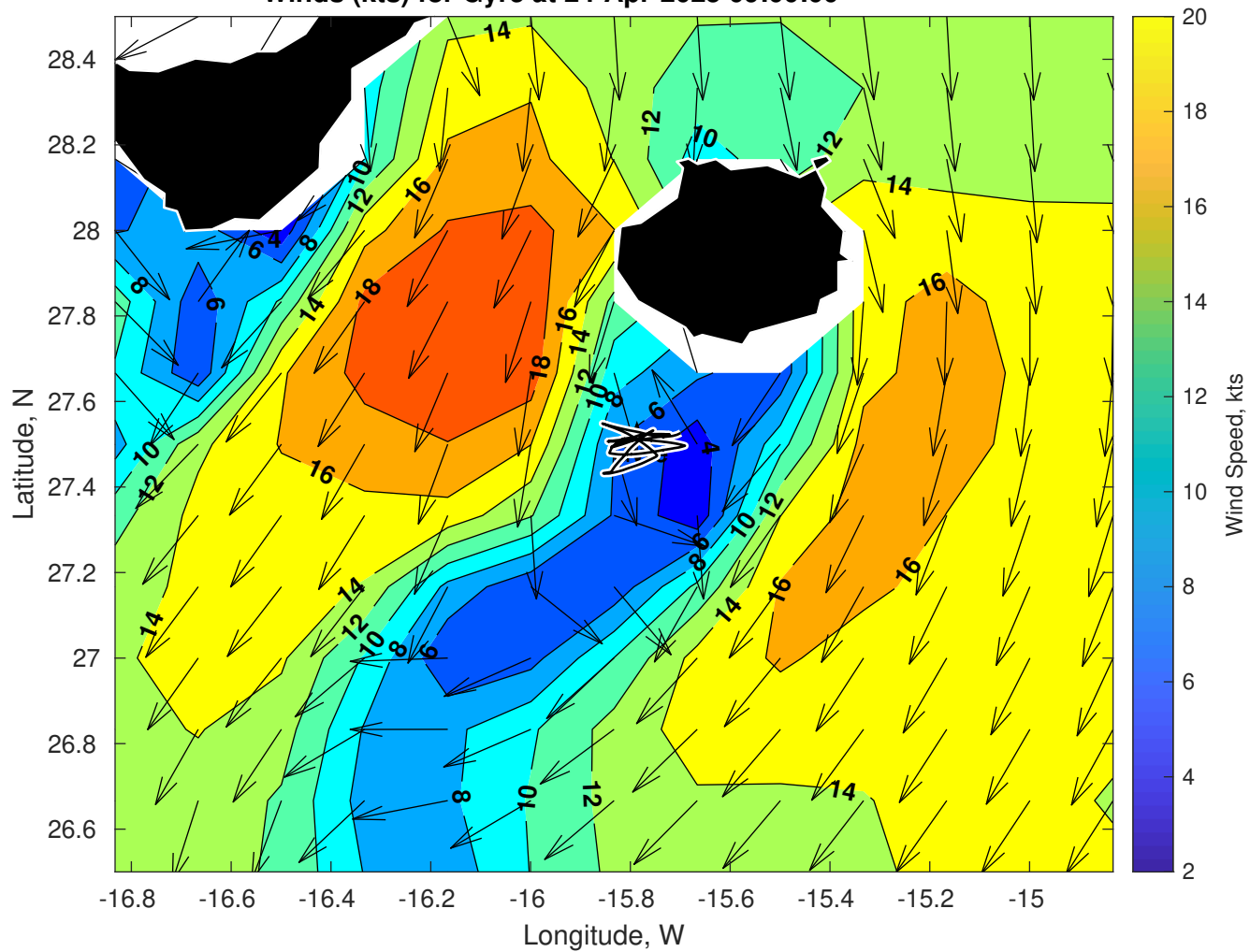
Winds (kts) for Gyre at 24-Apr-2025 09:00:00
