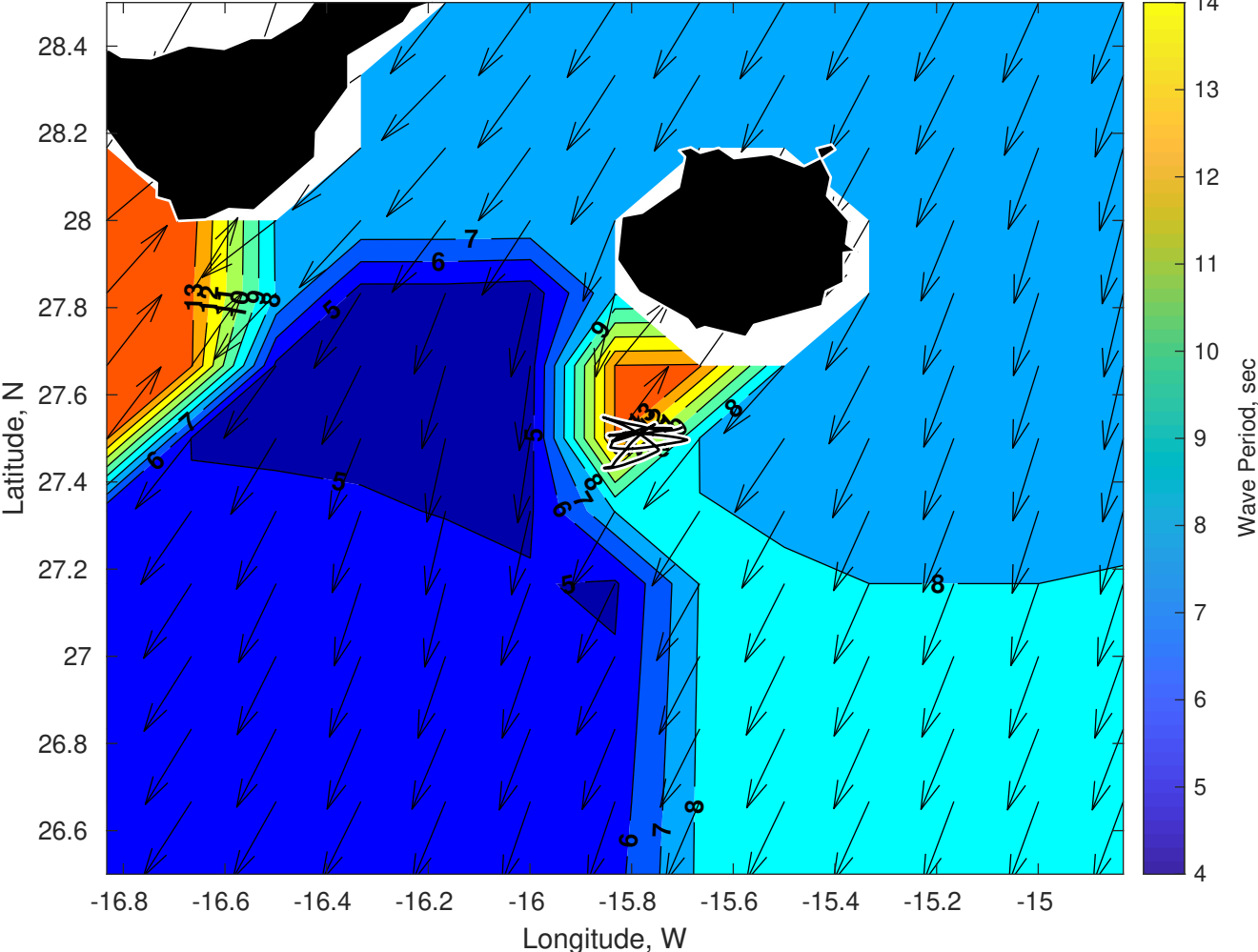
Wave Period (sec) for Gyre at 24-Apr-2025 09:00:00
