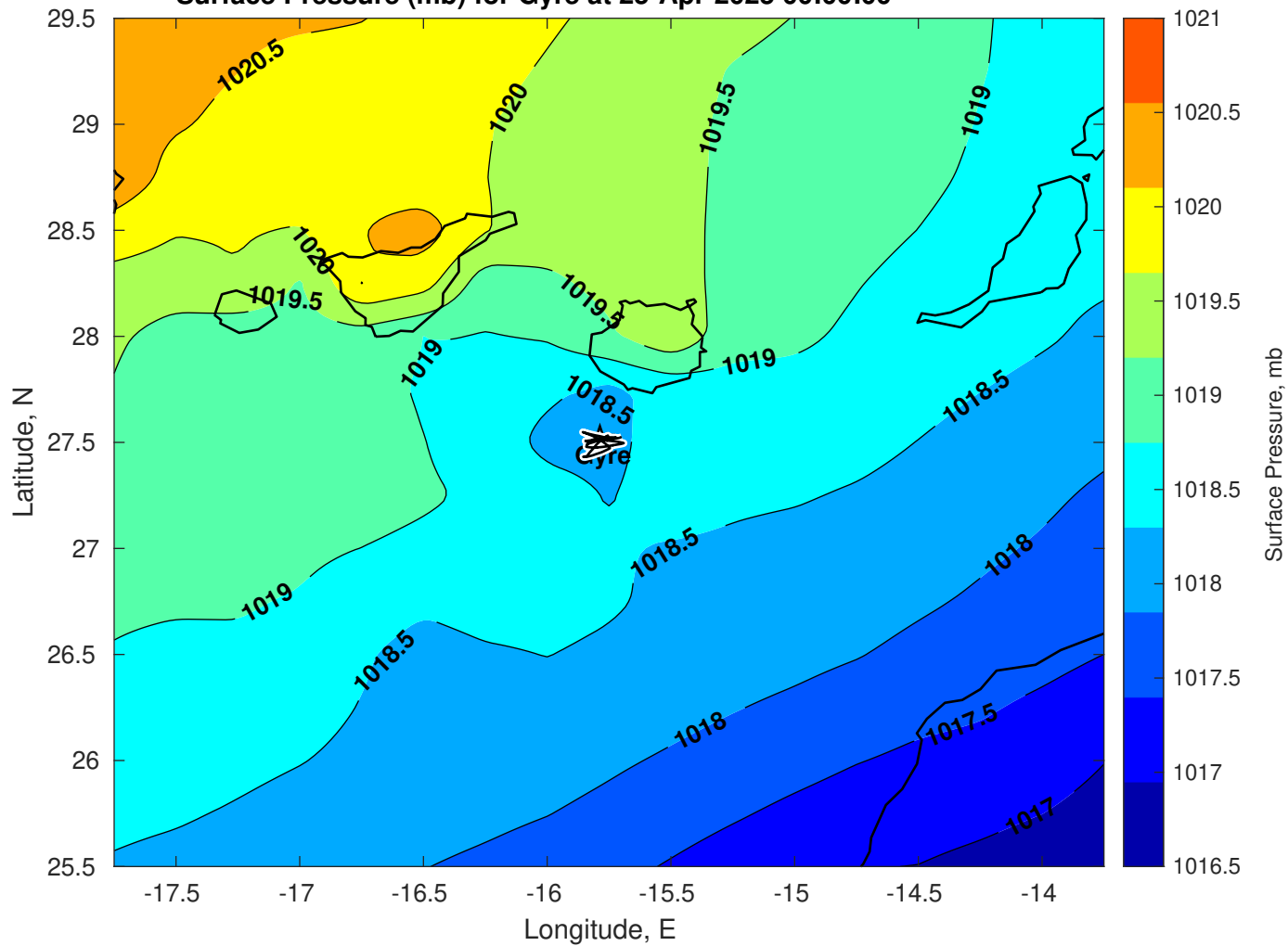
Surface Pressure (mb) for Gyre at 25-Apr-2025 00:00:00
