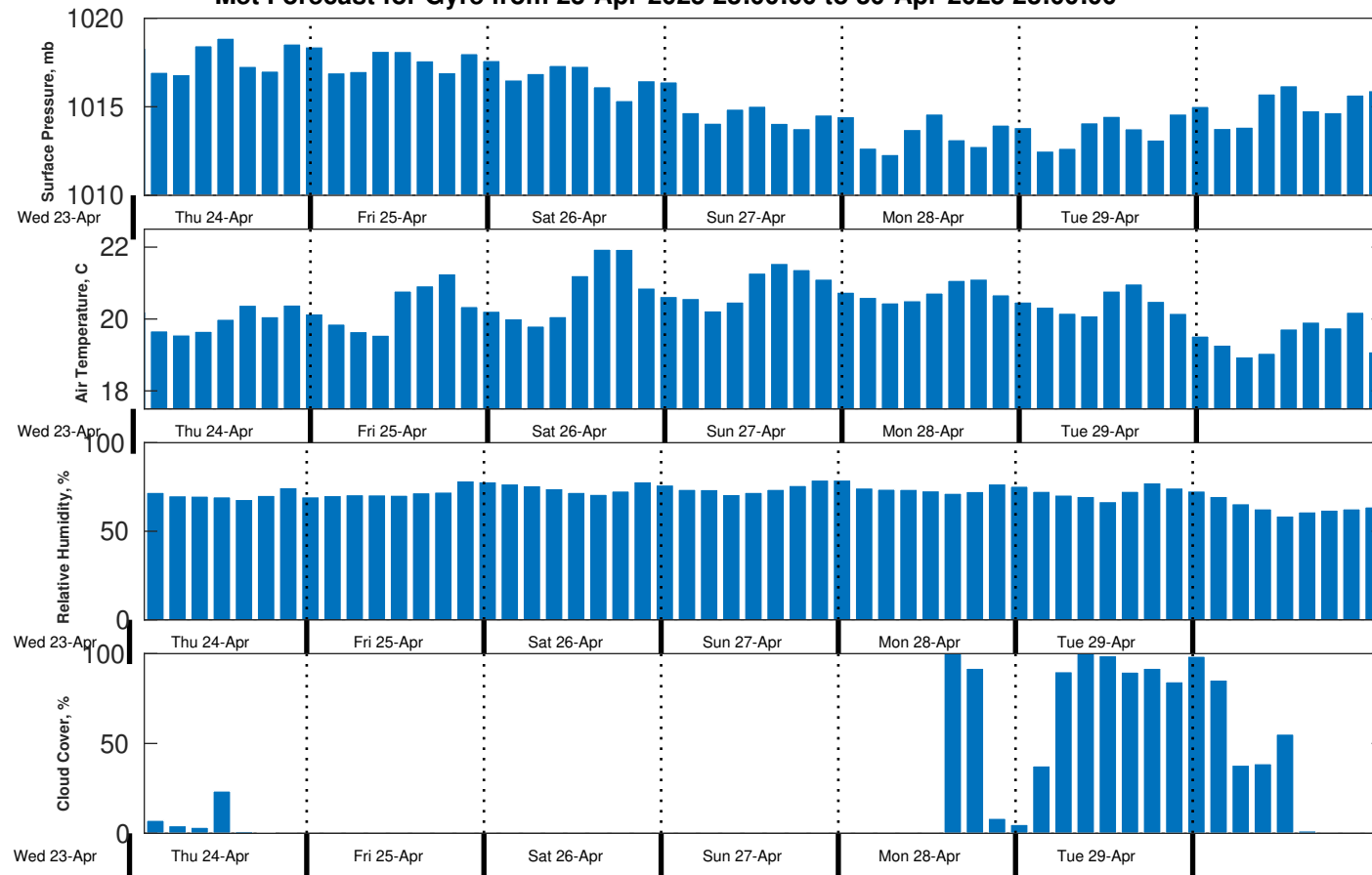
Met Forecast for Gyre from 23-Apr-2025 23:00:00 to 30-Apr-2025 23:00:00
