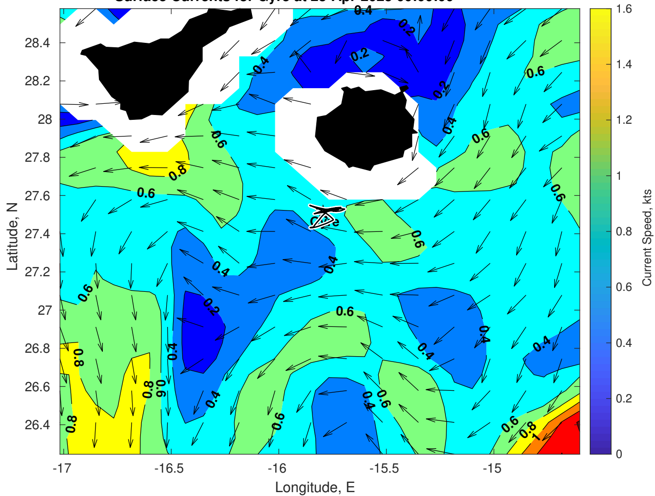
Surface Currents for Gyre at 23-Apr-2025 00:00:00
