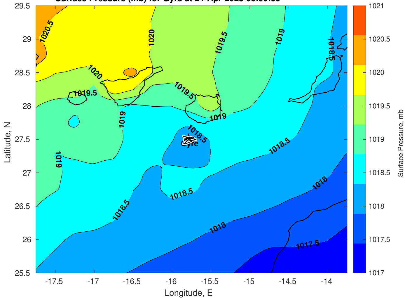
Surface Pressure (mb) for Gyre at 24-Apr-2025 00:00:00
