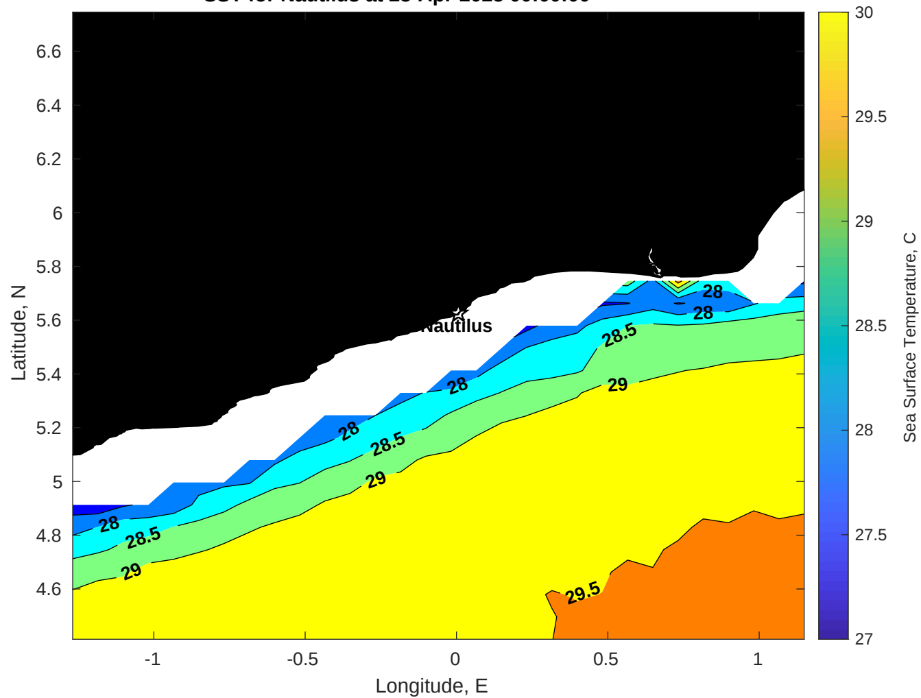
SST for Nautilus at 23-Apr-2025 00:00:00
