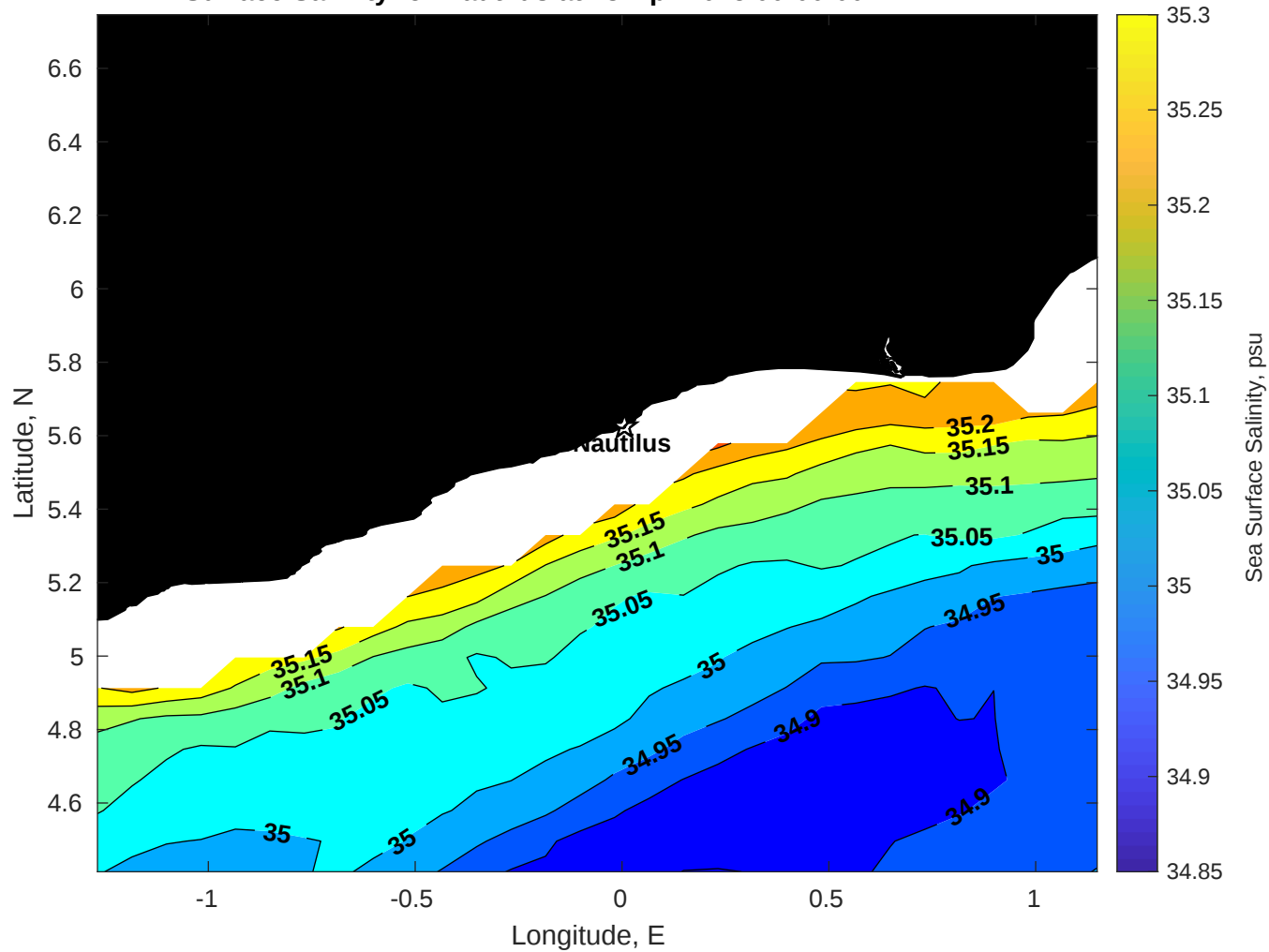
Surface Salinity for Nautilus at 23-Apr-2025 00:00:00
